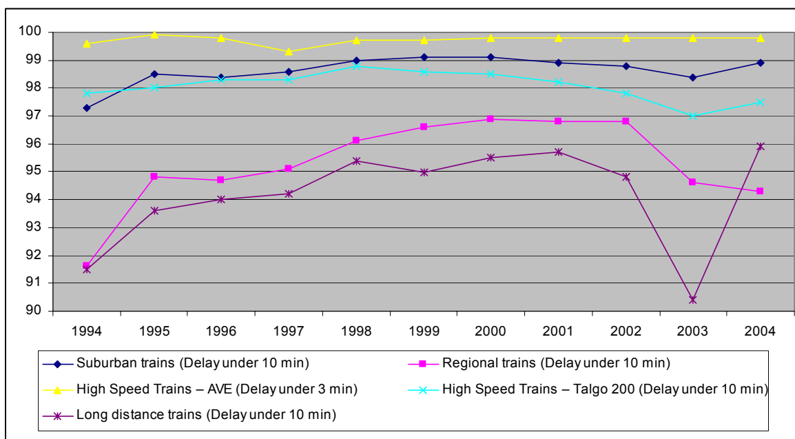
Figure 7-9: RENFE: percentage of punctual trains evolution Source: own elaboration from RENFE annual reports and accounts
