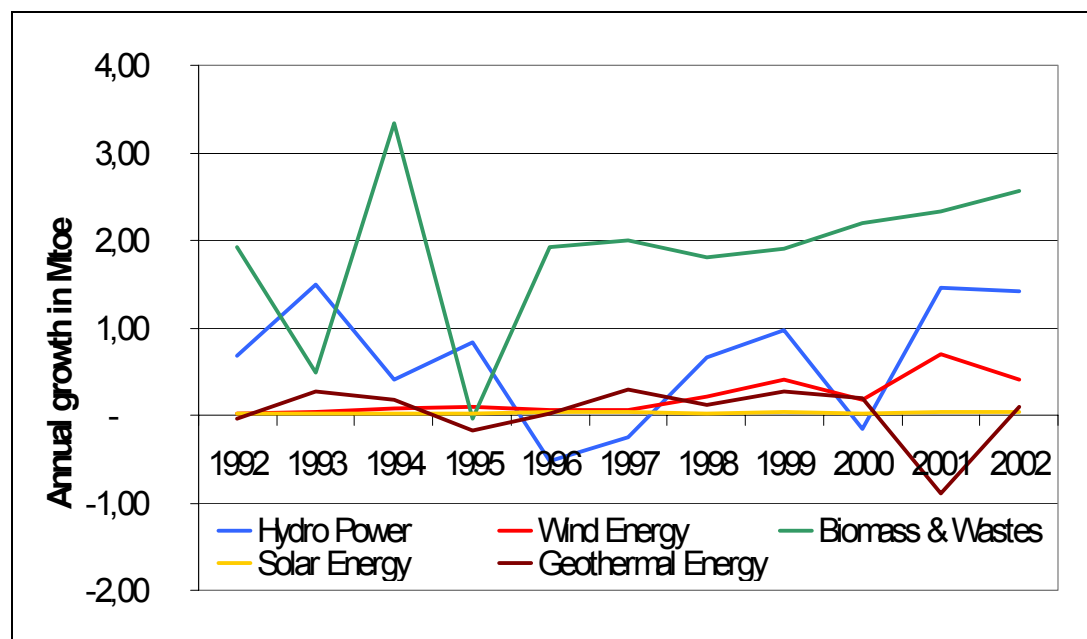
Figure A.2.3: The annual growth rate of RES
