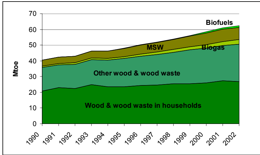
Figure A.2.4: Gross energy consumption per type of biomass
