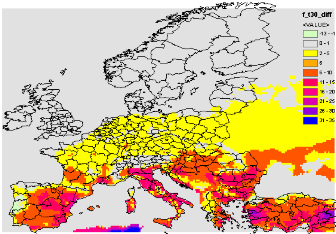
Map A.15 Heat days (Tmax>30°C) difference 1961 – 2009
