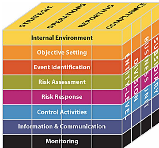
Figure 2 COSO framework
