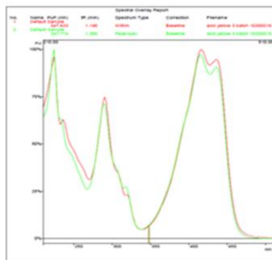
• DAD Spectra Overlay for the dye Acid Yellow 3 in disulfonated and monosulfonated form
