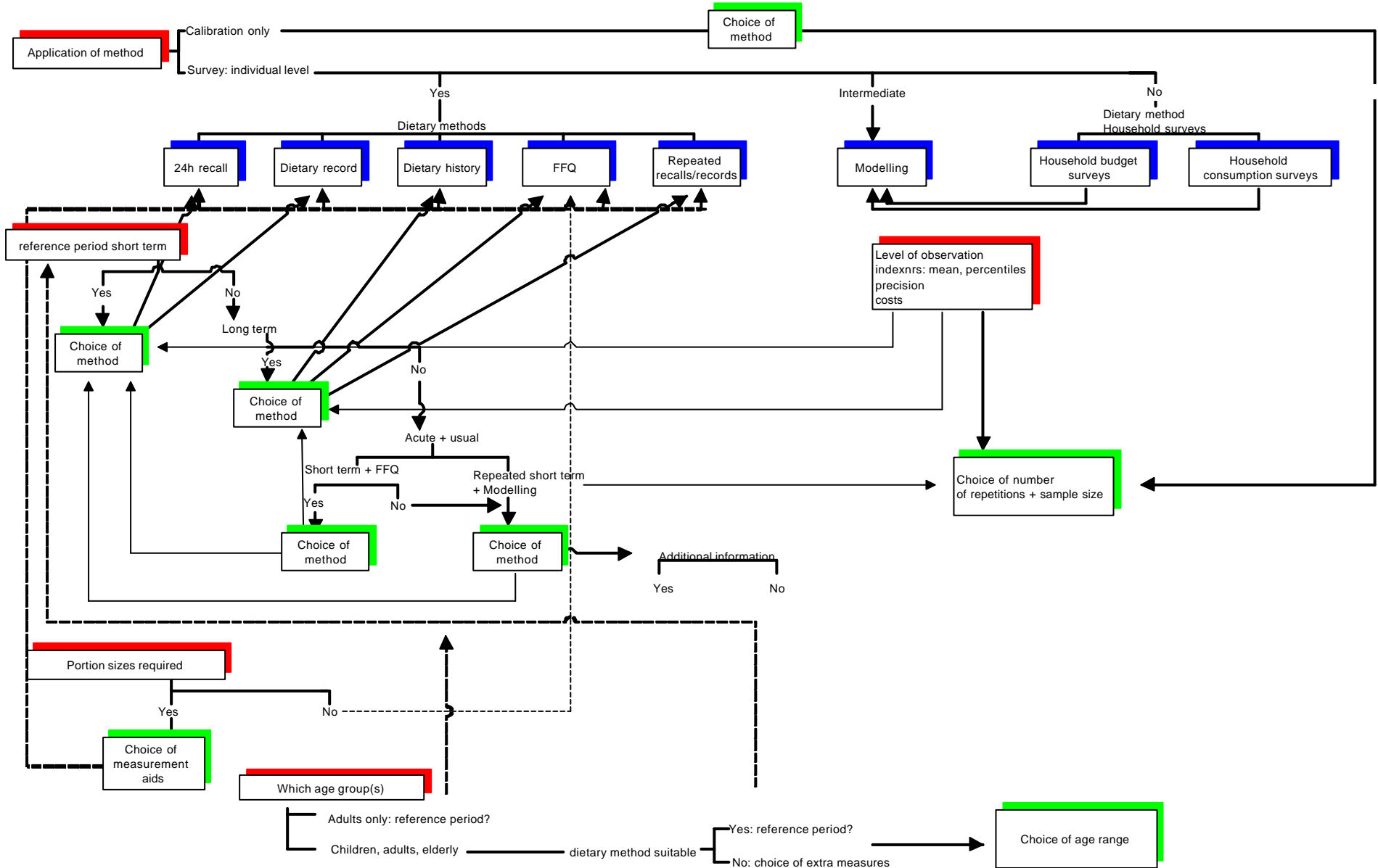
Figure 2 Decision tree: methods and sample size (green = moments of choice; blue = alternatives; red = criteria)
