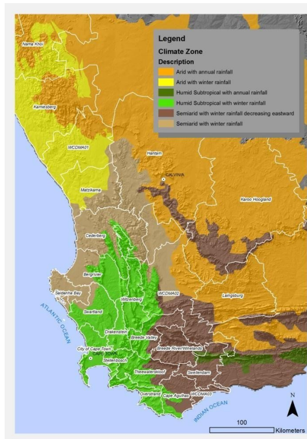
Figure 2: A description of the climate of the south-western part of South Africa with the aid of Köppen classes (Source: Western Cape Department of Agriculture)
