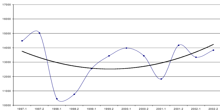
Figure 1: EU 15 gross indigenous production from the first half of 1997 to the second half of 2002
