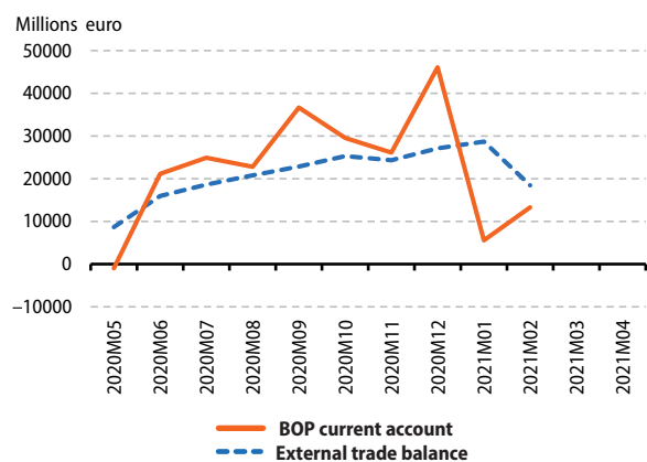
Figure 5: External transactions
