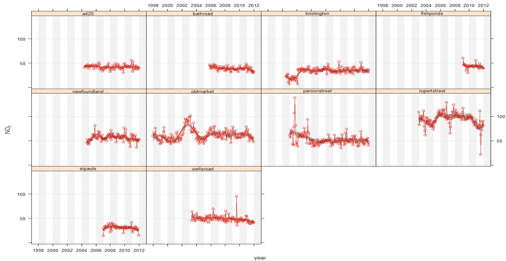
Figure 3 Trends in annual mean nitrogen dioxide concentration ( \mu\text{gm}^{-3} ) measured at automatic monitoring sites
