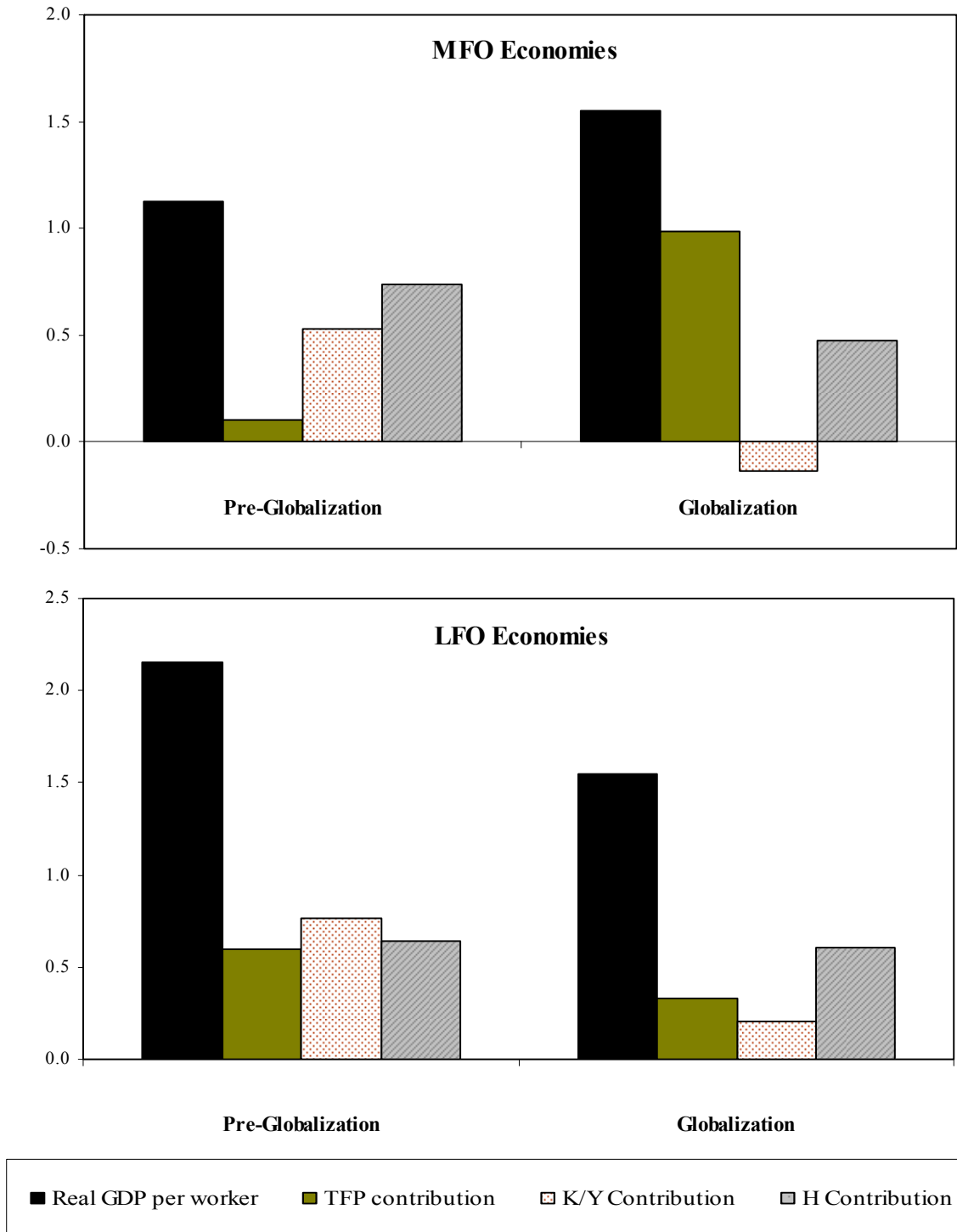
Figure 2. Growth Accounting for More and Less Financially Open Economies (De Facto Measure of Financial Integration. Constant Sample)
