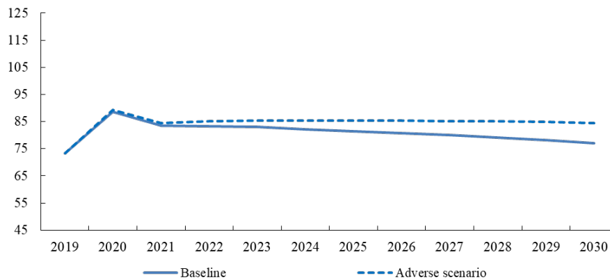
Graph 2. General government debt (% of GDP)
