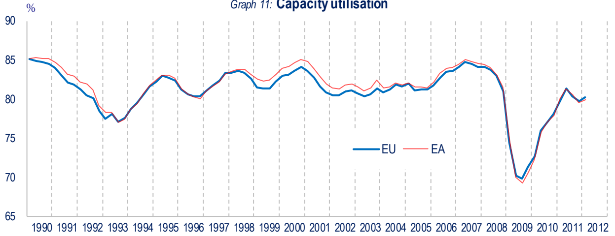
Graph 11: Capacity utilisation
