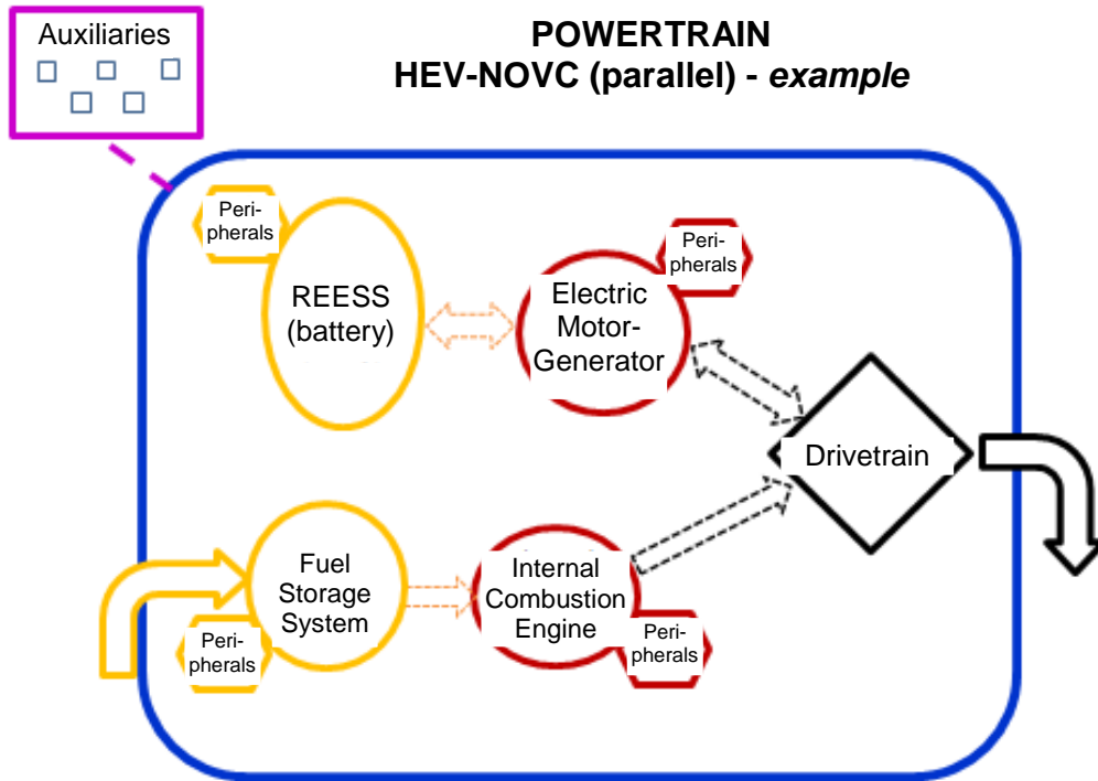
Figure 4 Hybrid Electric Vehicle-Not Off Vehicle Charging (parallel) - HEV-NOVC
