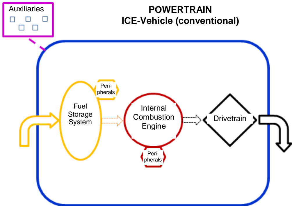
Figure 2 Internal Combustion Engine-Vehicle (conventional) - ICEV
