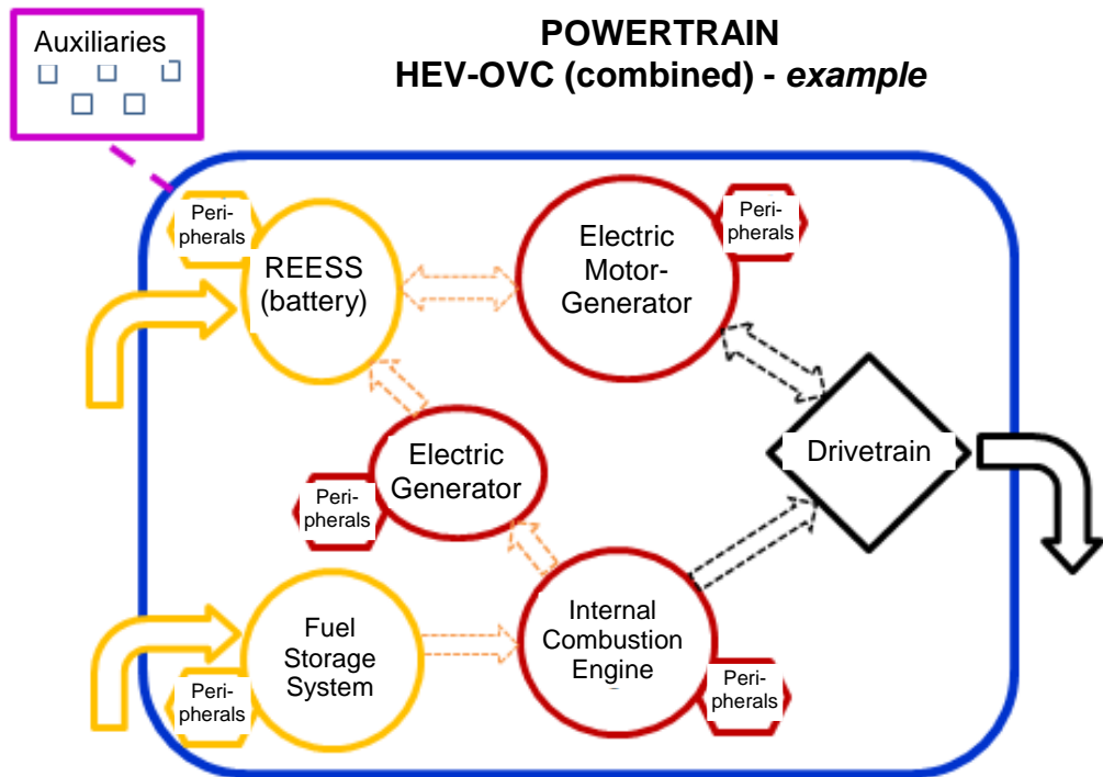
Figure 6 Hybrid Electric Vehicle-Off Vehicle Charging (combined) - HEV-OVC
