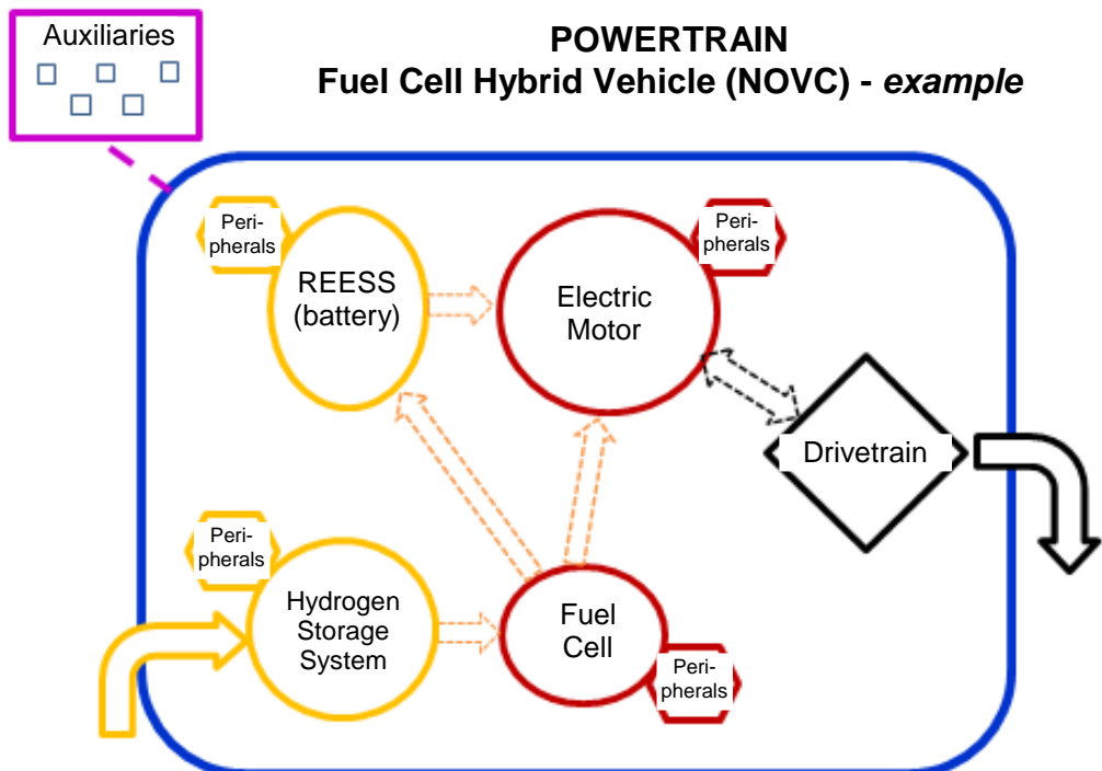
Figure 7 Fuel Cell Hybrid Vehicle (Not Off Vehicle Charging) - FCHV-NOVC
