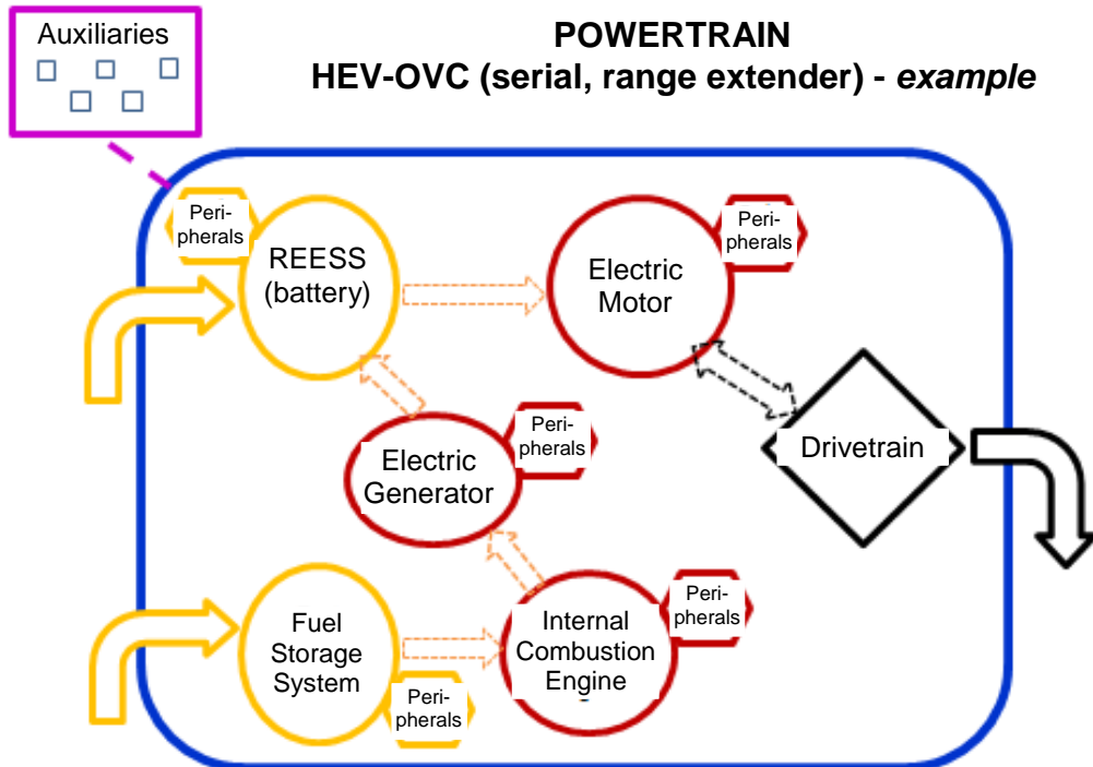
Figure 5 Hybrid Electric Vehicle-Off Vehicle Charging (serial, range extender) - HEV-OVC
