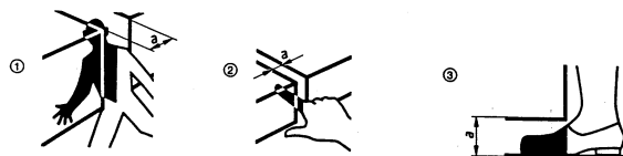
Figure 6 (Fig. A.1 from EN 349)
