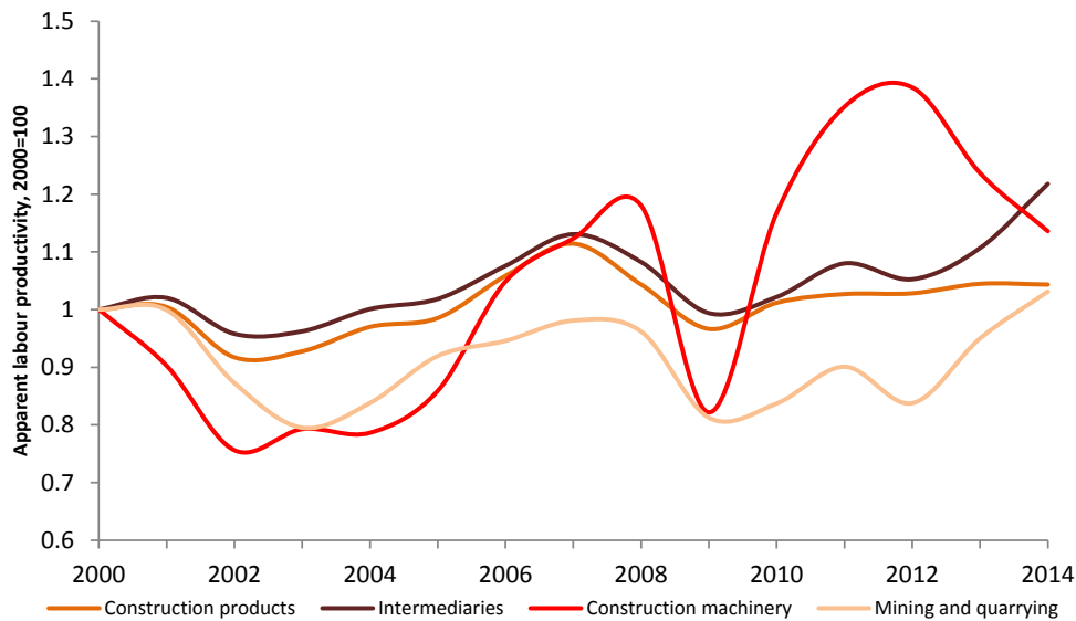
Figure 32: Apparent labour productivity in the CVC
