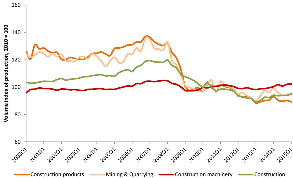
Figure 27 Changes in the volume of production in the CVC 46 (index 100 = in 2010)
