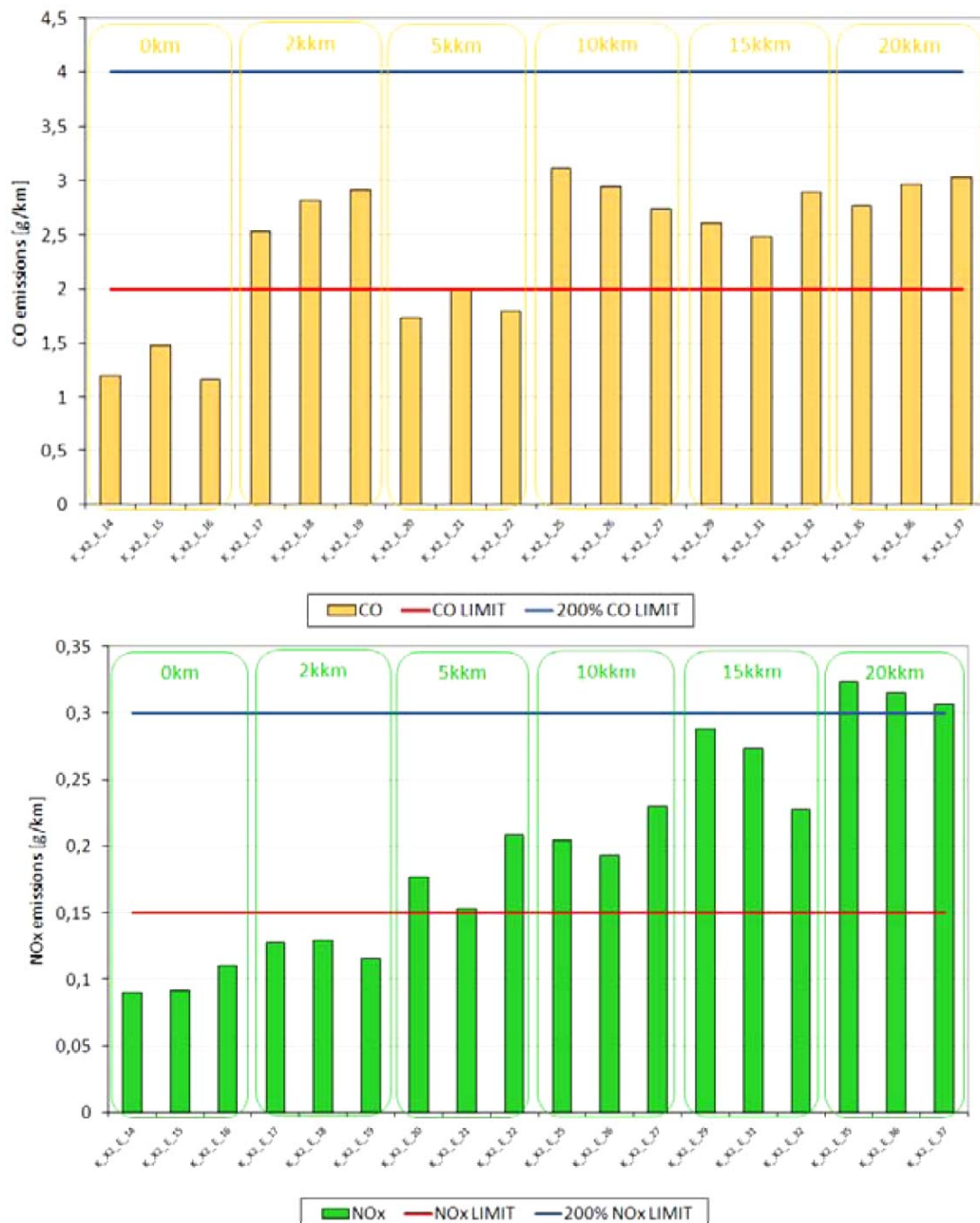
Figure 3-13: Results of the 2008 AECC Motorcycle Test Program of AECC on one 500cc scooter run for about 20000 km
