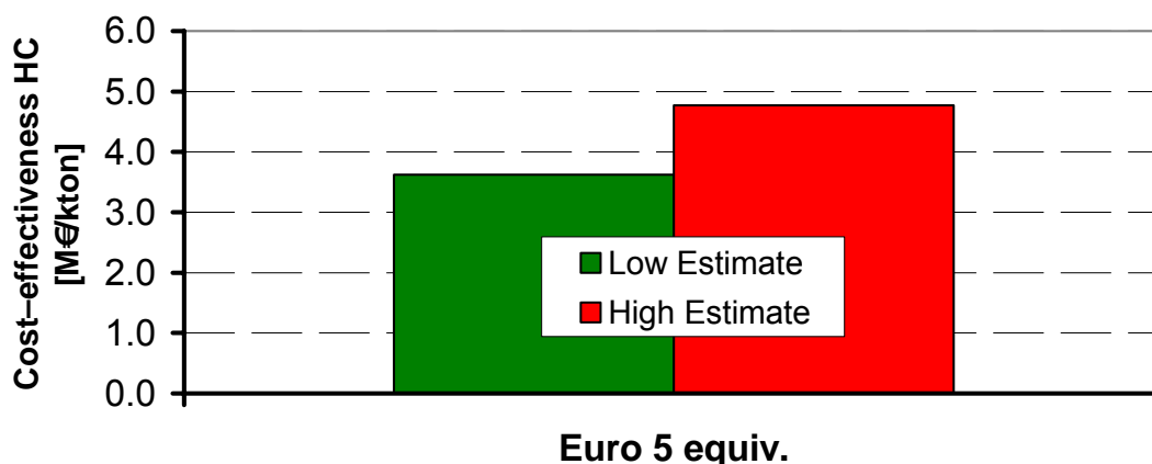
Figure 3-16: HC cost effectiveness for IUC of motorcycles.
