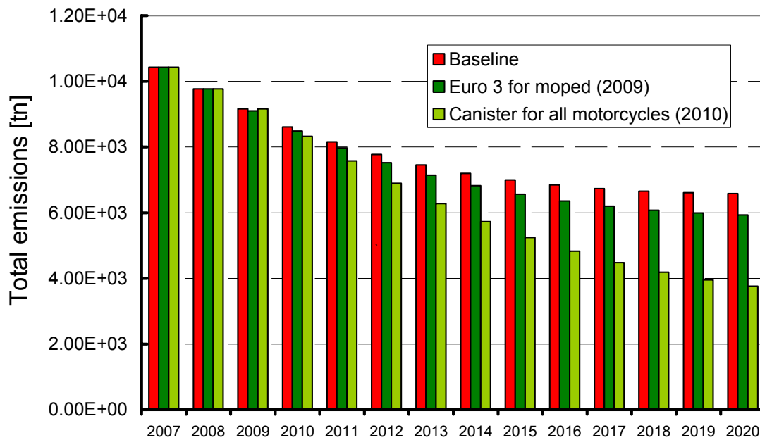
Figure 3-24: Evolution of the total evaporative emissions for the examined scenarios
