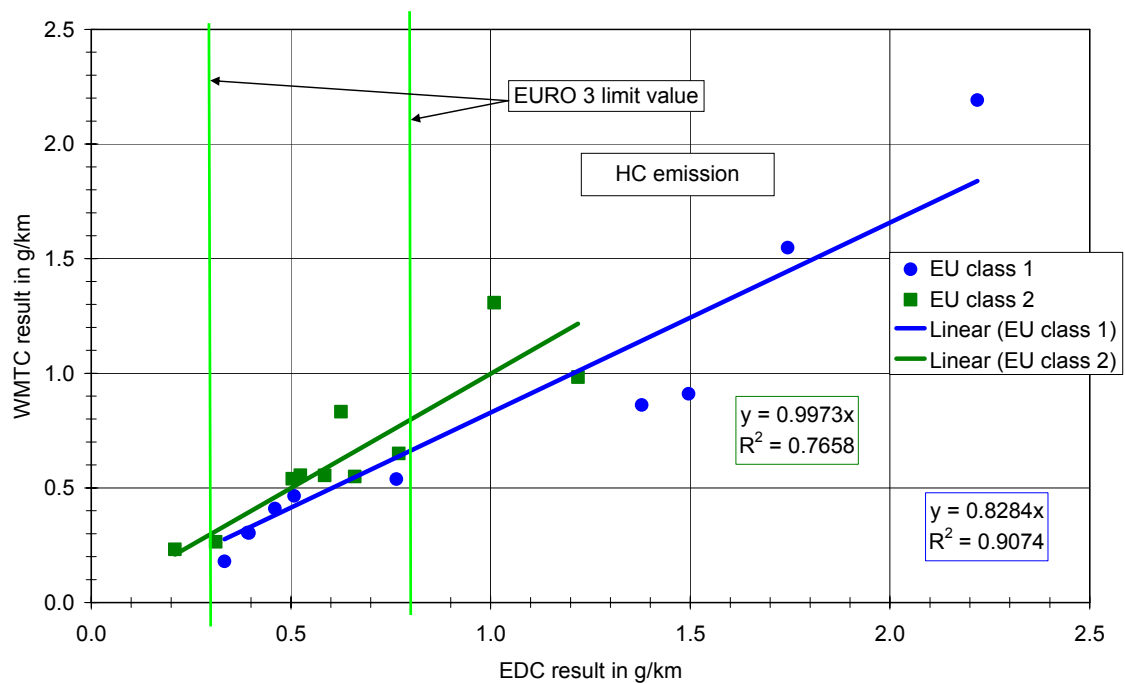
Figure 4-14: WMTC cycle results versus 2002/51/EC cycle (6 UDC (+ EUDC) cold) results for HC, WMTC class 2
