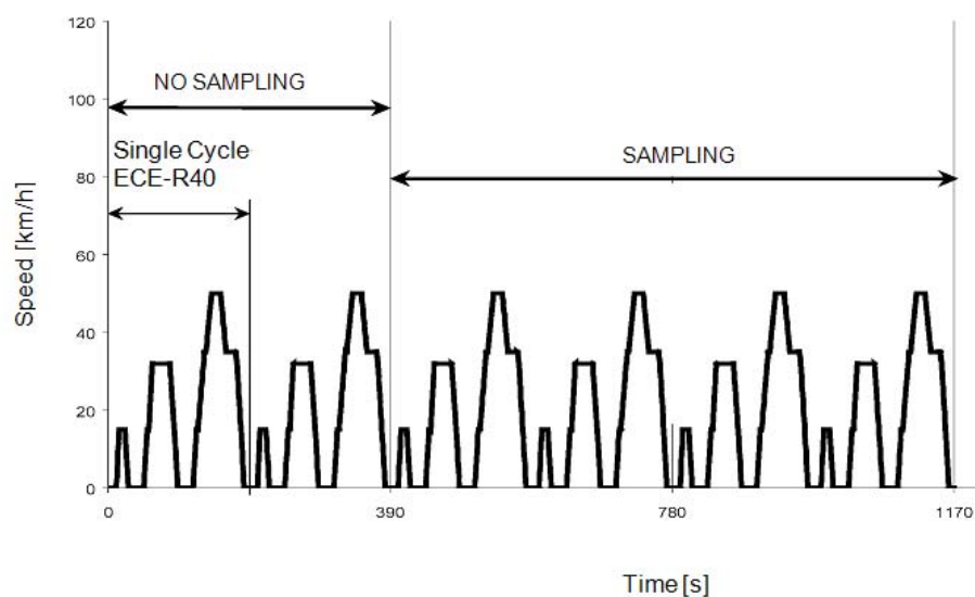
Figure 2-10: ECE-R40, Driving cycle for motorcycles (Euro 1 and Euro 2). Pollutant sampling is conducted after the first two subcycle repetitions
