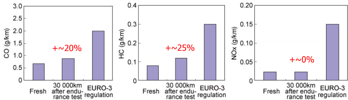
Figure 3-12: Results on durability from a 1100 cc Honda Motorcycle (Honda R&D Co, SAE Paper 2004-32-0032)
