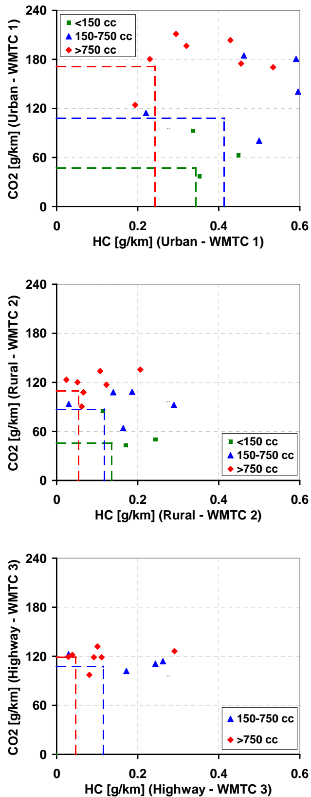
Figure 2-19: Derivation of emission factors for Best Available Technology (CO 2 vs HC)
