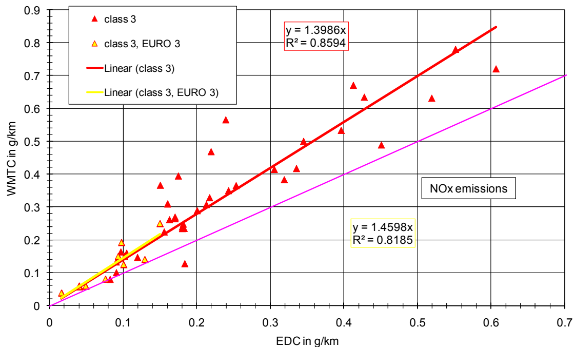
Figure 4-18: WMTC cycle results versus 2002/51/EC cycle (6 UDC + EUDC cold) results for NO x , WMTC class 3
