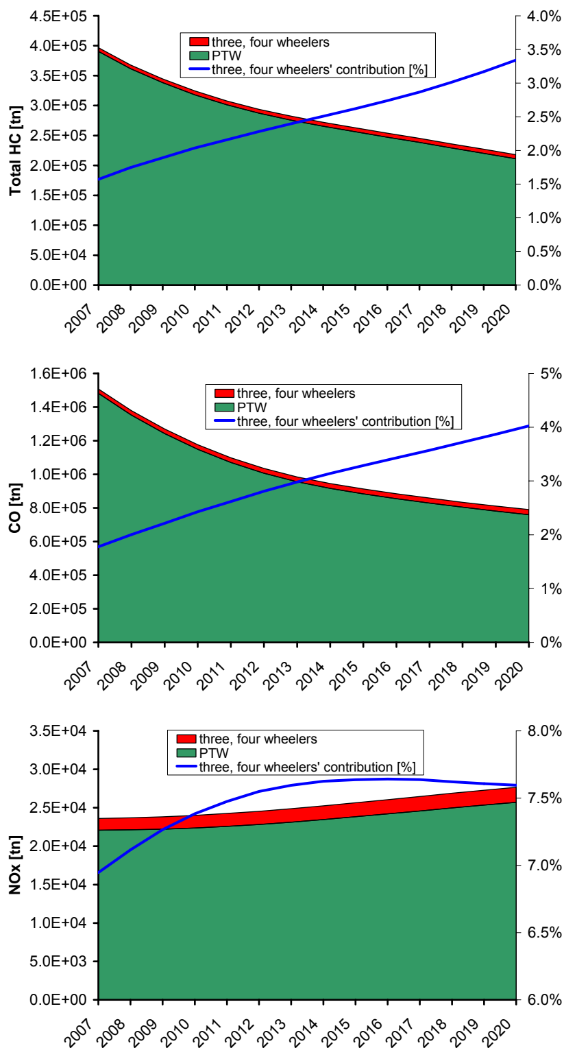
Figure 3-2: Evolution of emissions of 3 & 4 wheelers and comparison with total motorcycle emissions. top: total HC (exhaust & evaporation, middle: CO, bottom: NO x .
