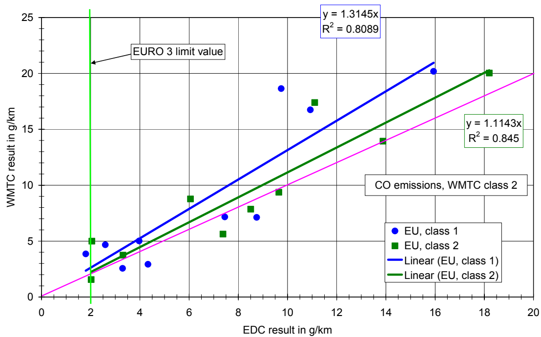
Figure 4-13: WMTC cycle results versus 2002/51/EC cycle (6 UDC (+ EUDC) cold) results for CO, WMTC class 2
