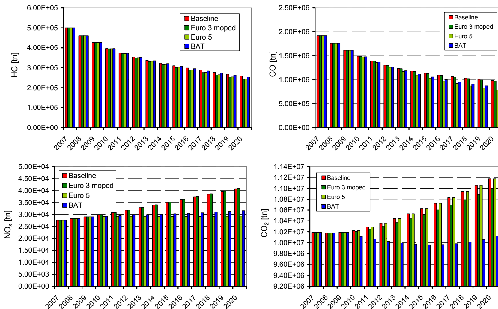
Figure 3-3: Estimated evolution of regulated pollutants from total PTWs in EU15 due to the introduction of different emission standards
