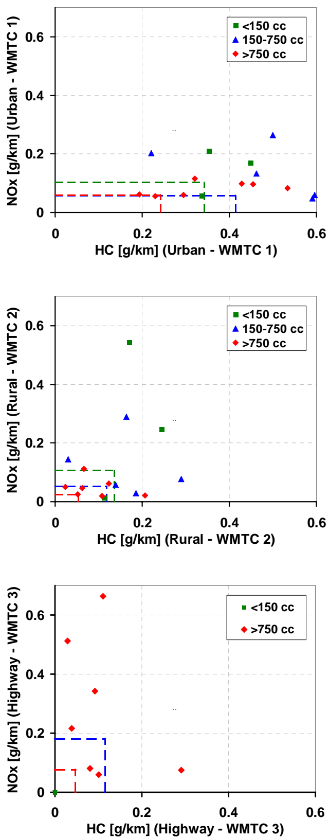
Figure 2-18: Derivation of emission factors for Best Available Technology (NO x vs HC)
