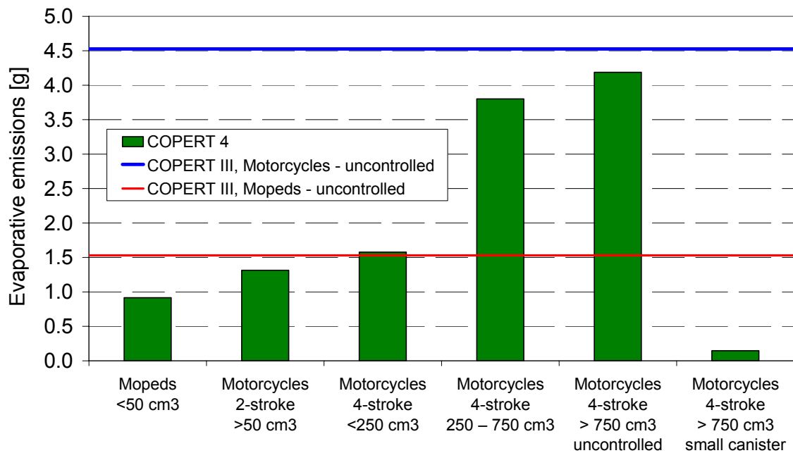
Figure 2-20: Example of typical daily evaporative emissions estimated with COPERT III and COPERT 4 methodology
