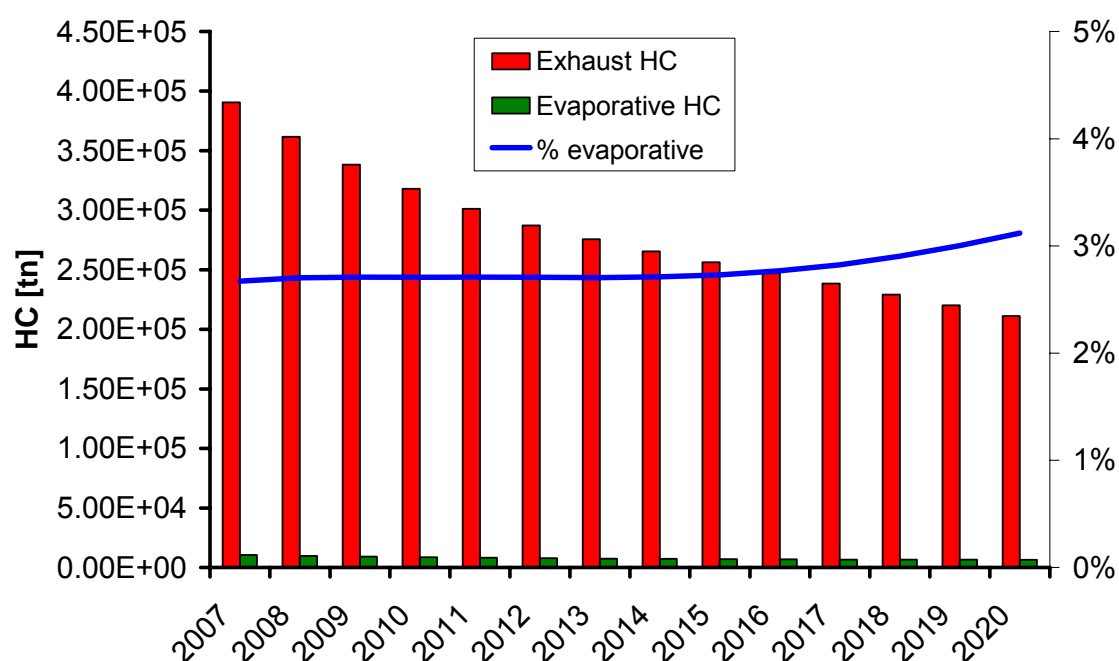
Figure 3-23: Evolution of exhaust and evaporative HC emissions from motorcycles and % contribution of evaporative losses to total HC emissions for the baseline scenario
