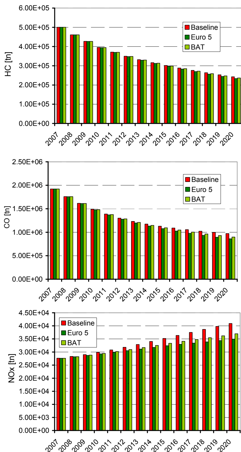
Figure 3-19: Estimated evolution of regulated pollutants from total PTWs in EU15 due to the introduction of different OBD requirements
