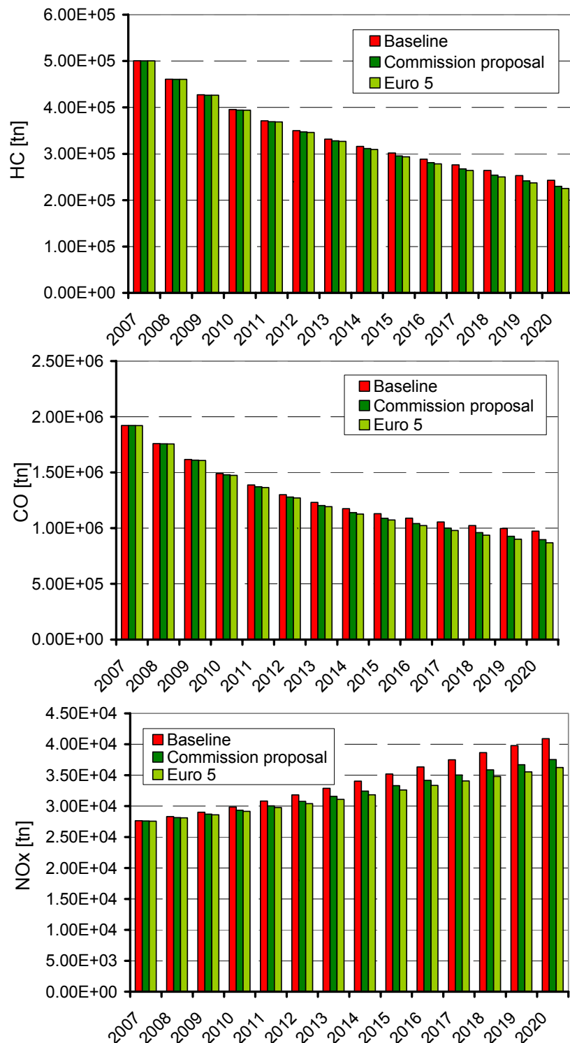
Figure 3-10: Estimated evolution of regulated pollutants from total PTWs in EU15 due to the introduction of different durability requirements
