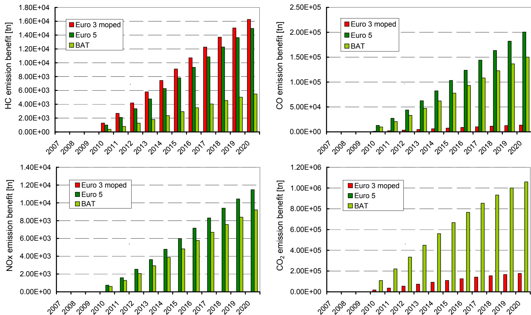
Figure 3-4: Estimated emission benefit evolution of regulated pollutants from total PTWs in EU15 due to the introduction of different emission standards
