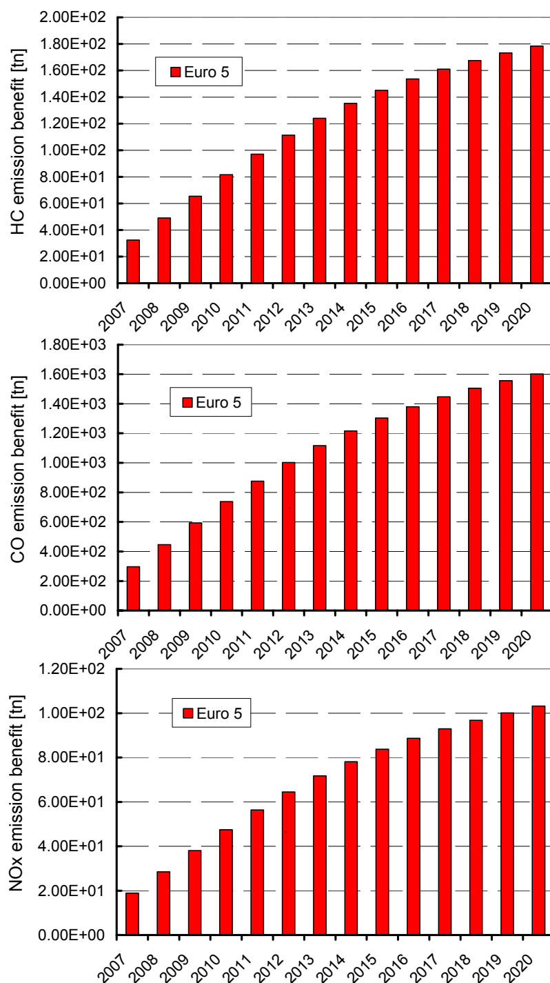
Figure 3-15: Estimated emission benefit of regulated pollutants from total PTWs in EU15 due to the introduction of In Use Compliance requirements
