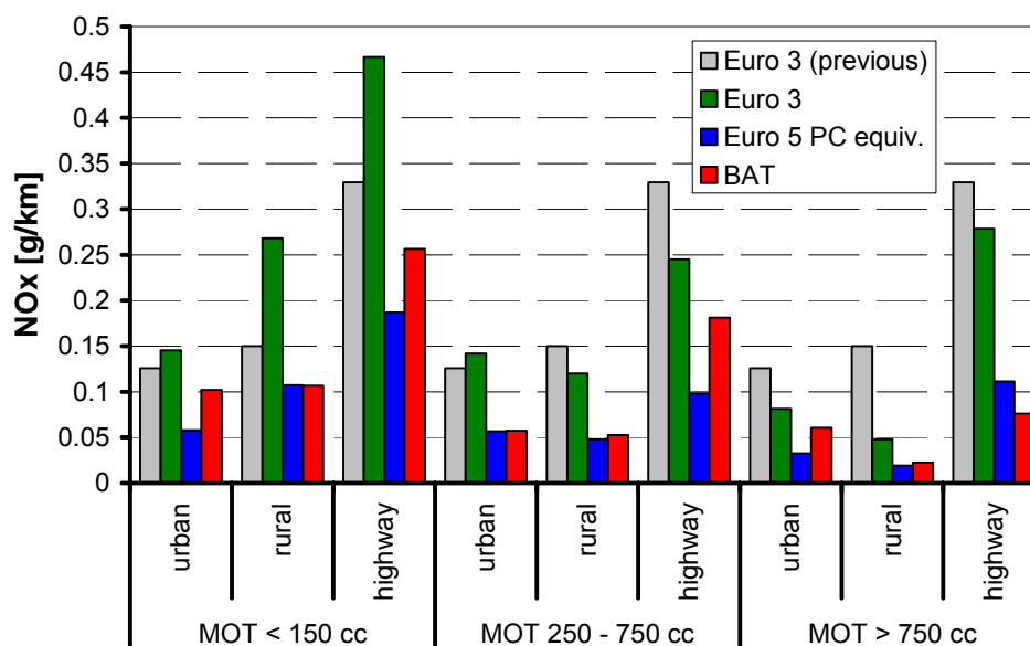
Figure 2-15: Updated NOx emission factors for Euro 3 and post Euro 3 technology assumptions
