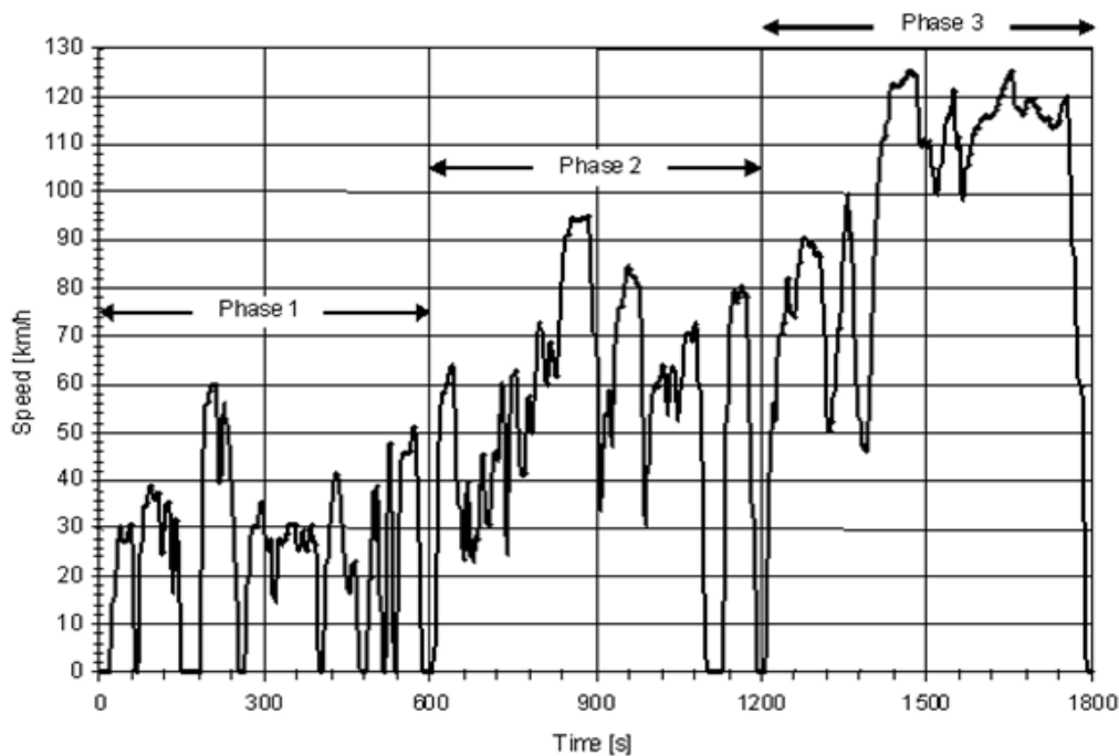
Figure 2-12: WMTc, alternative driving cycle for the type-approval of Euro 3 motorcycles.
