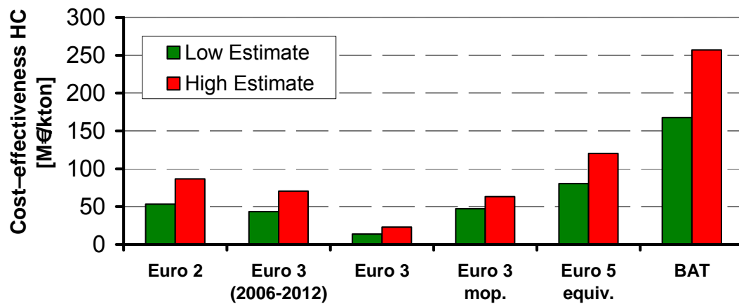
Figure 3-6: HC cost effectiveness for different PTW emission standards
