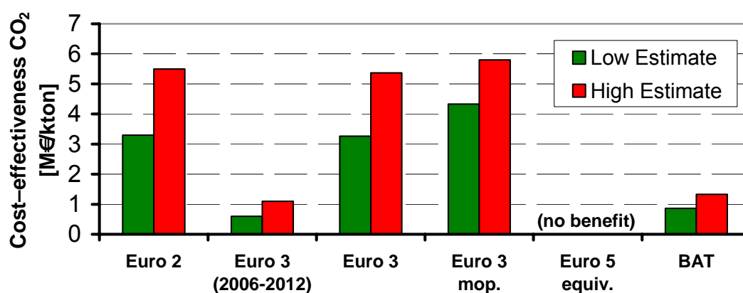
Figure 3-9: CO 2 cost effectiveness for different PTW emission standards
