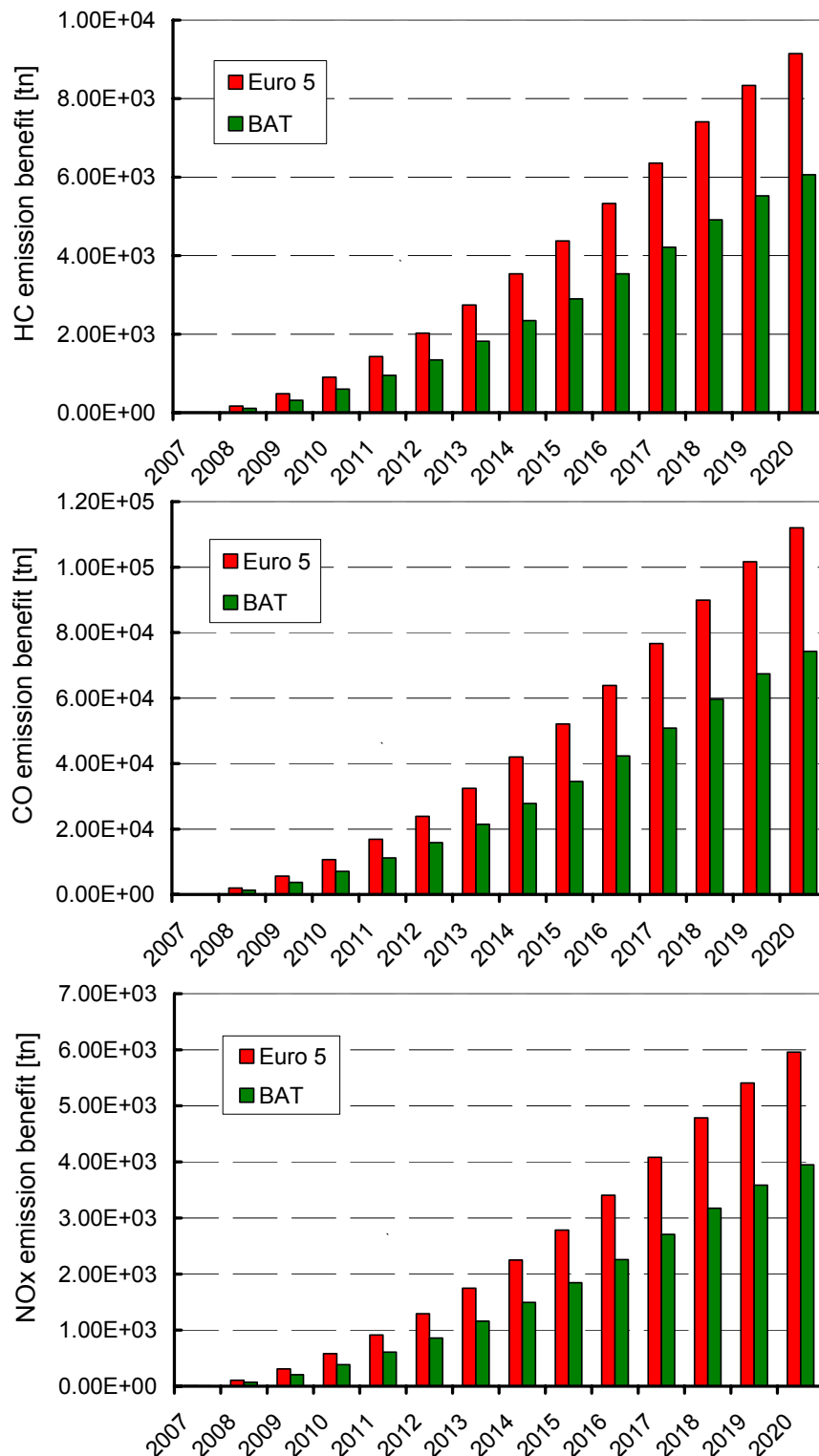
Figure 3-20: Estimated emission benefit of regulated pollutants from total PTWs in EU15 due to the introduction of different OBD requirements.
