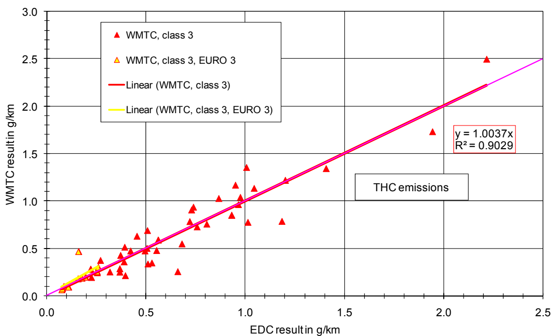
Figure 4-20: WMTC cycle results versus 2002/51/EC cycle (6 UDC + EUDC cold) results for HC, WMTC class 3
