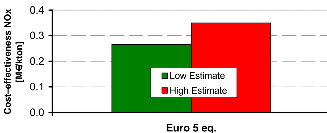
Figure 3-17: NO x cost effectiveness for IUC of motorcycles.
