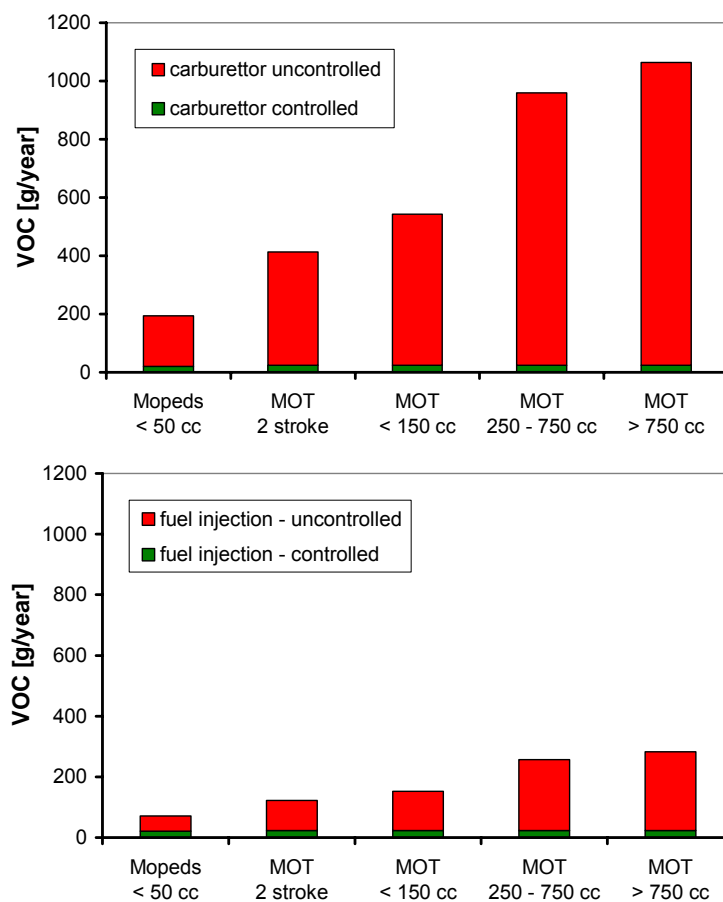
Figure 2-21: Typical annual emissions of HC due to evaporation, as a function of vehicle category and emission control technology.
