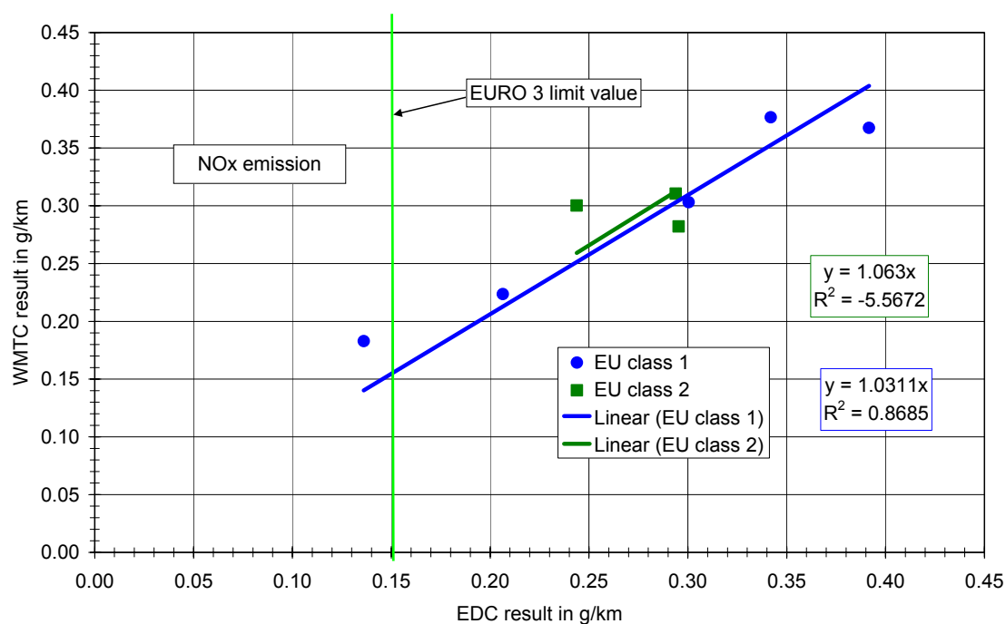
Figure 4-15: WMTC cycle results versus 2002/51/EC cycle (6 UDC + EUDC cold) results for NO x , WMTC class 2 without high CO emitters
