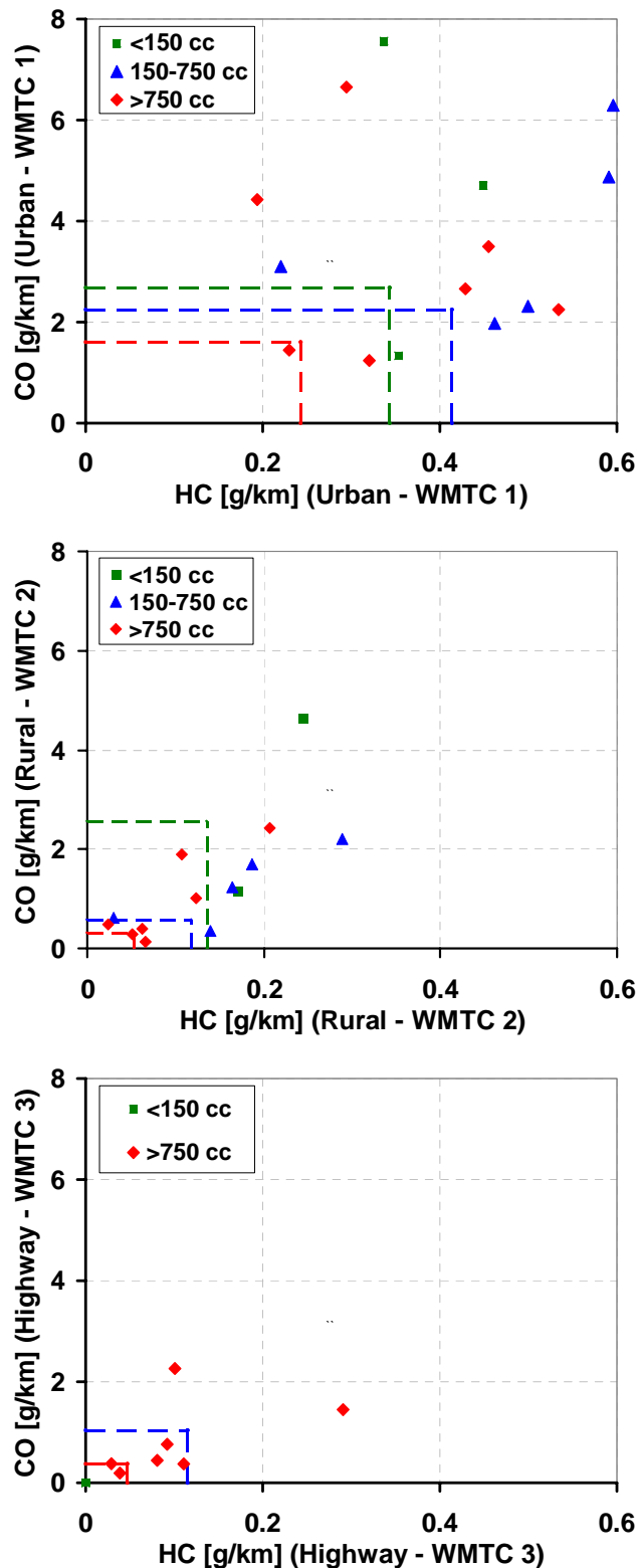
Figure 2-17: Derivation of emission factors for Best Available Technology (CO vs HC)
