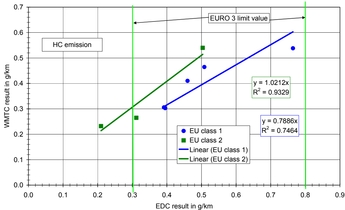
Figure 4-17: WMTC cycle results versus 2002/51/EC cycle (6 UDC + EUDC cold) results for HC, WMTC class 2 without high CO emitters
