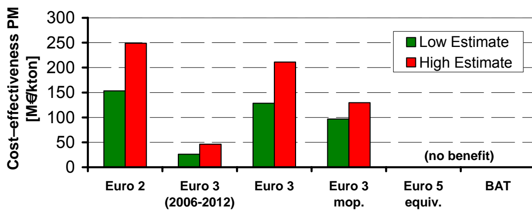
Figure 3-8: PM cost effectiveness for different PTW emission standards
