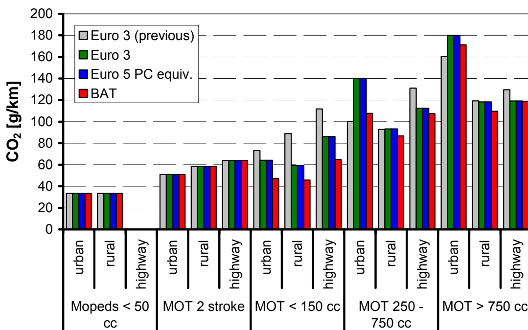
Figure 2-16: Updated CO 2 emission factors for Euro 3 and post Euro 3 technology assumptions
