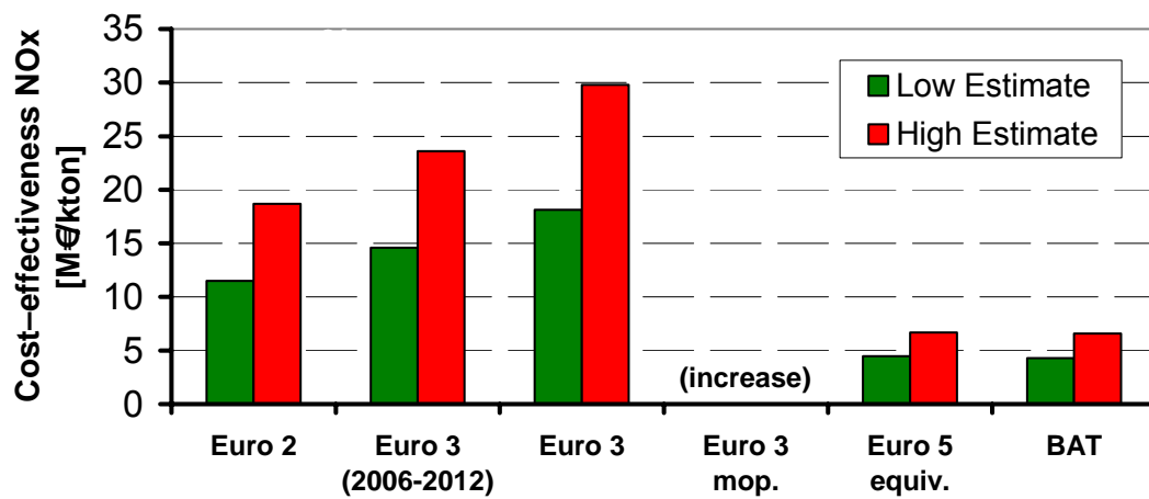
Figure 3-7: NO x cost effectiveness for different PTW emission standards
