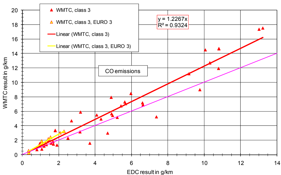
Figure 4-19: WMTC cycle results versus 2002/51/EC cycle (6 UDC + EUDC cold) results for CO, WMTC class 3
