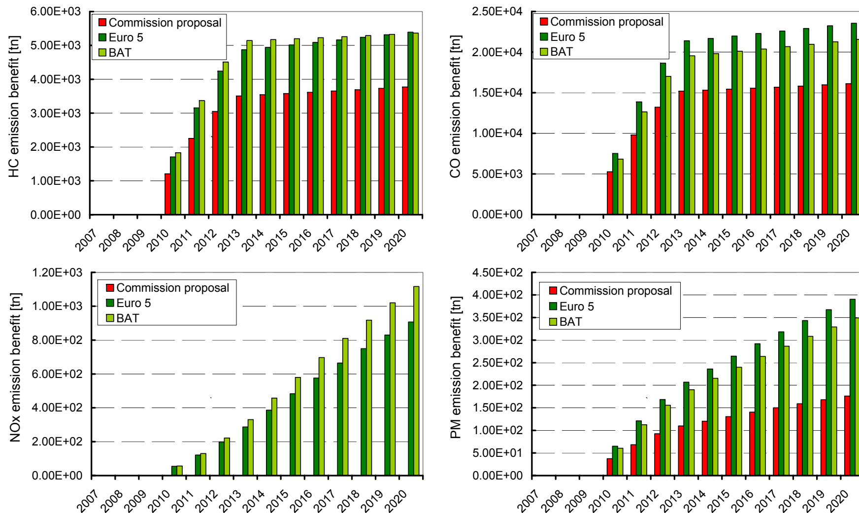
Figure 3-28: Estimated emission benefit of regulated pollutants and PM from tri- and quadricycles in EU15 due to the introduction of different emission standards
