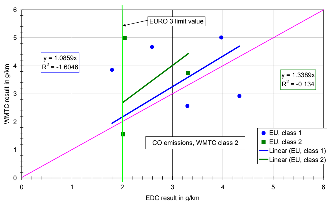
Figure 4-16: WMTC cycle results versus 2002/51/EC cycle (6 UDC + EUDC cold) results for CO, WMTC class 2 without high CO emitters
