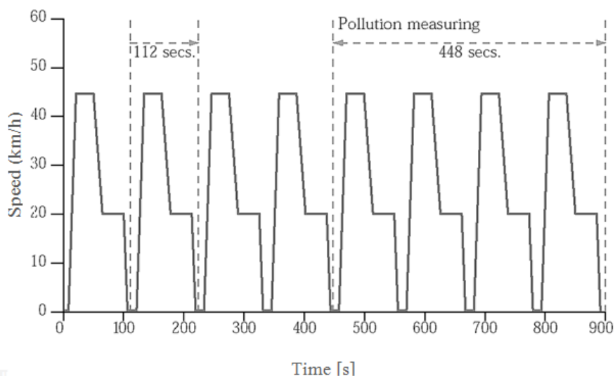
Figure 2-9: ECE-R47, Driving cycle for mopeds (Euro 1 and Euro 2). Pollutant sampling is conducted after the first four subcycle repetitions.
