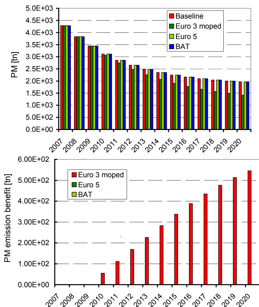
Figure 3-5: Estimated PM emissions (top) and PM emission benefit evolution (bottom) from total PTWs in EU15 due to the introduction of different emission standards.
