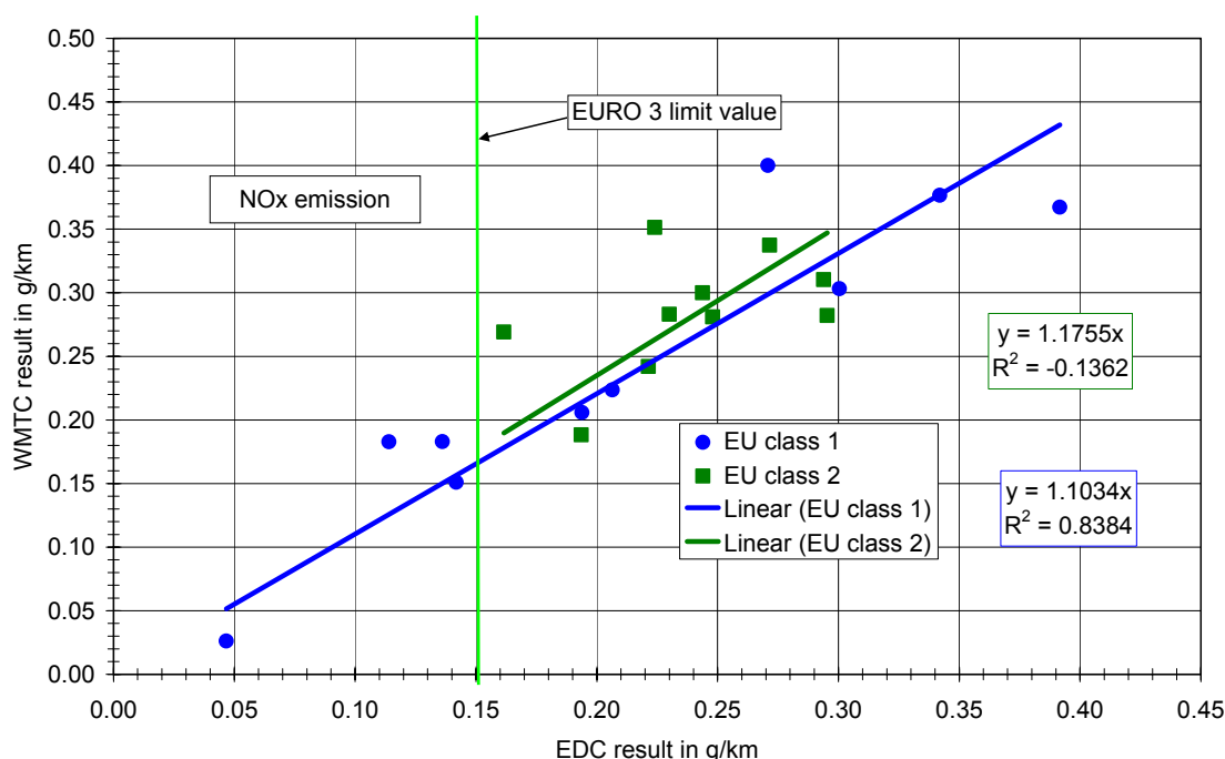
Figure 4-12: WMTC cycle results versus 2002/51/EC cycle (6 UDC (+ EUDC) cold) results for NOx, WMTC class 2
