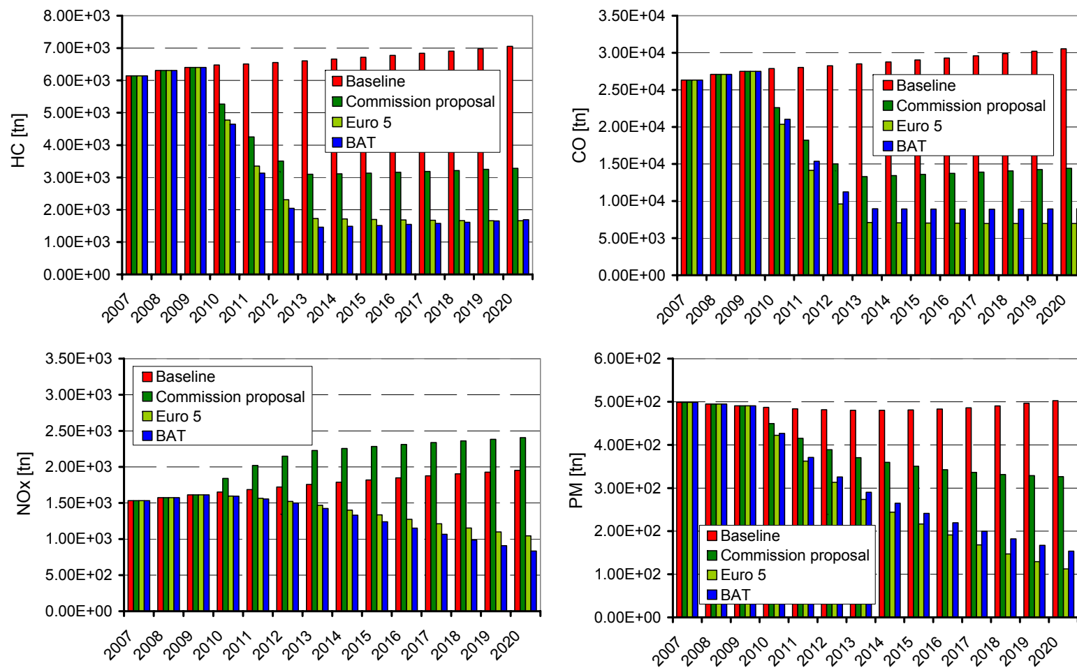
Figure 3-27: Estimated evolution of regulated pollutants and PM from tri- and quadricycles in EU15 due to the introduction of different emission standards
