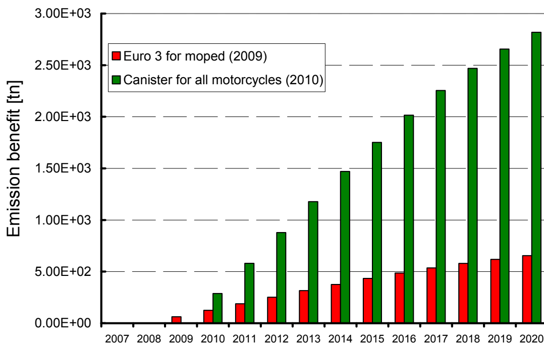
Figure 3-25: Total evaporative emissions benefit for the examined scenarios
