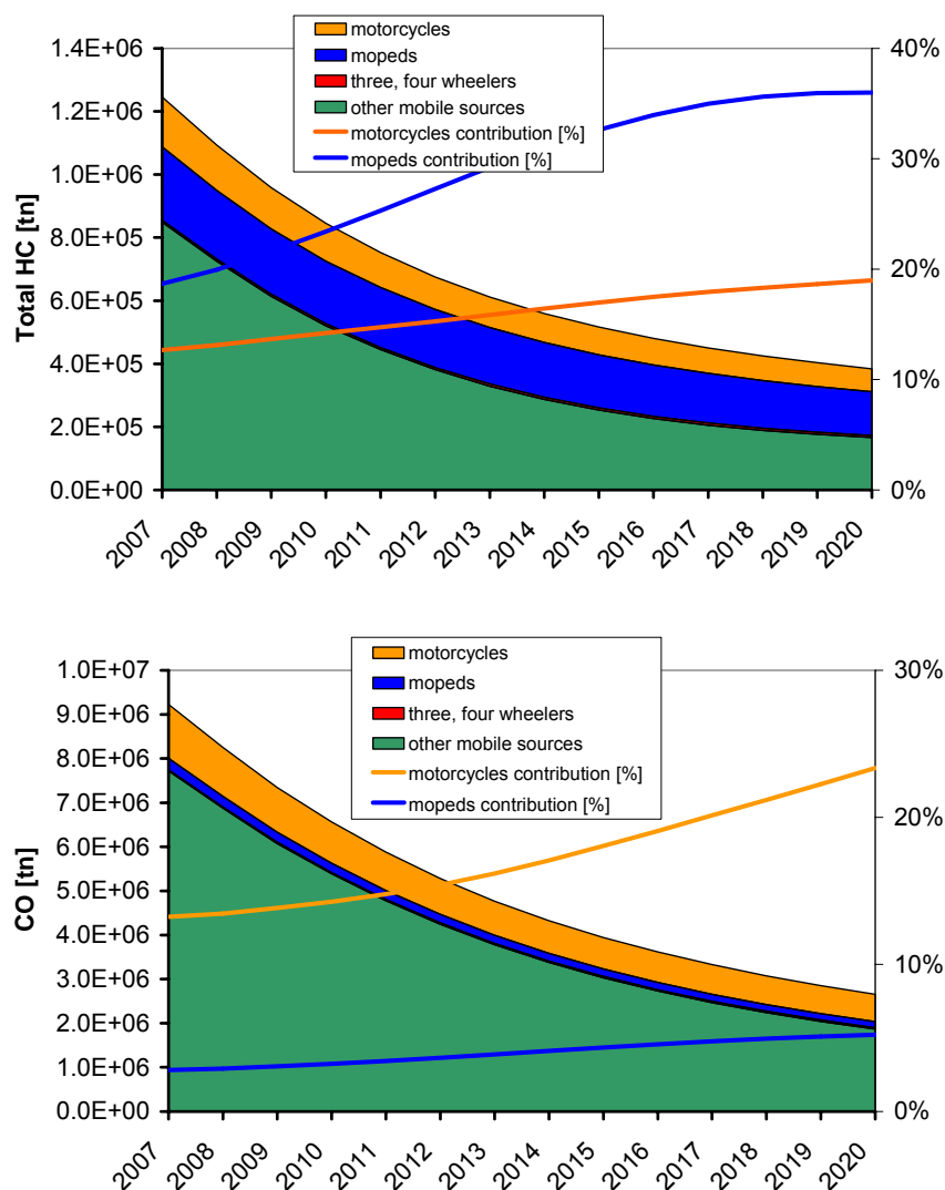
Figure 3-1: Evolution of PTW (incl. three and four wheelers) emissions according to the Baseline scenario. Comparison with emissions of all other road transport sources. top: total HC (exhaust & evaporation), bottom: CO
