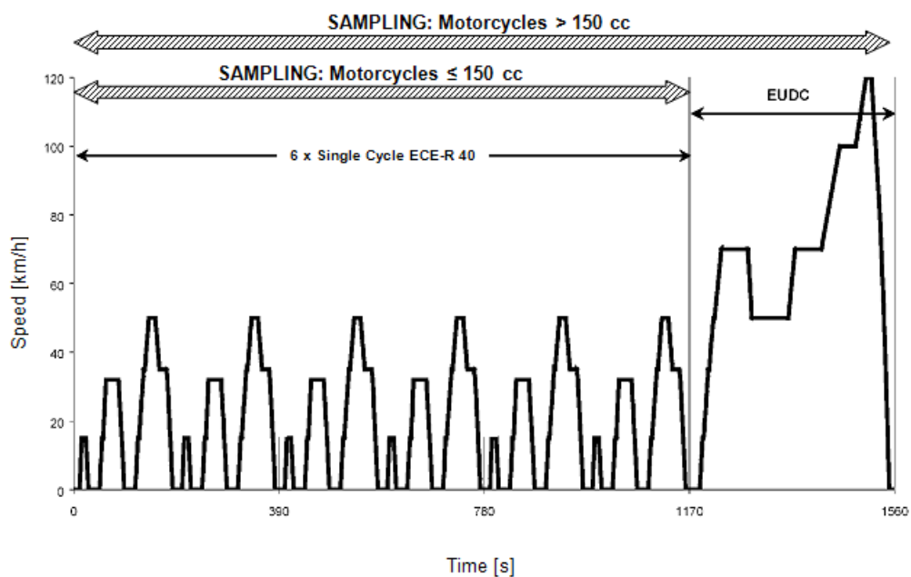
Figure 2-11: ECE-R40, cold (+EUDC) Driving cycle for motorcycles at a Euro 3 level. Only the cold ECE-R40 is used for motorcycles below or equal to 150 cc and the EUDC part is added for motorcycles of over 150 cc.
