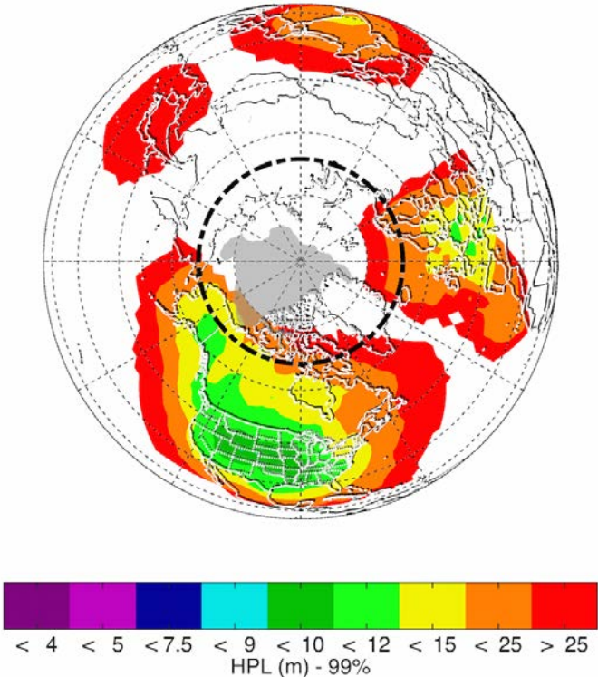
Figure 7: HPL for the Arctic Region Based on GPS L1 Augmented by WAAS + EGNOS + MSAS
