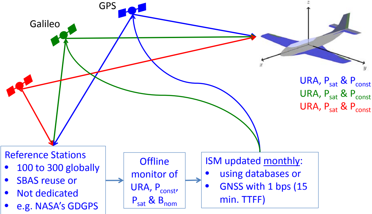
Figure 10: Offline V-ARAIM is based on the Ephemeris & Clock Data (ECD) Broadcast by the Core Constellations
