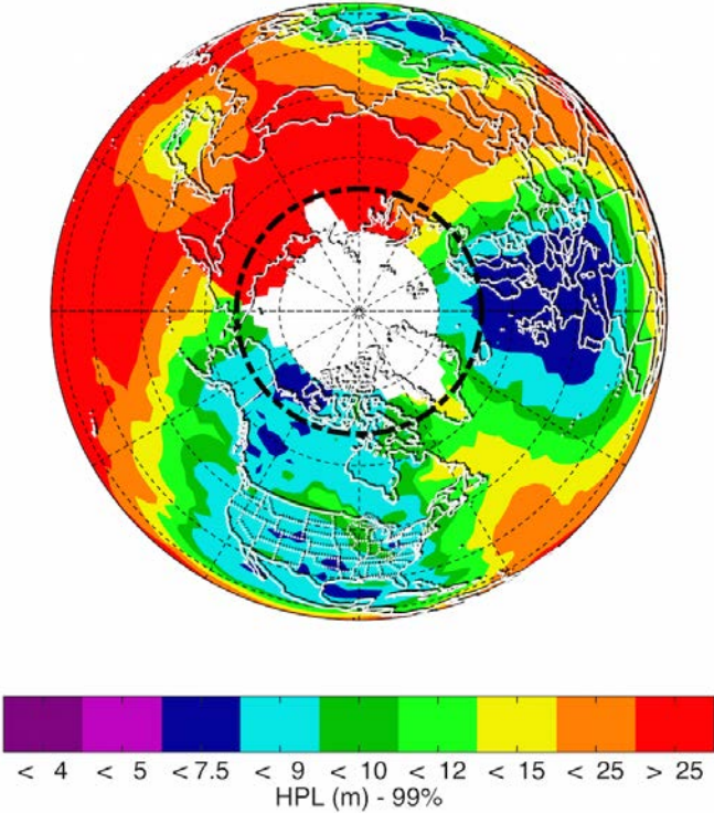
Figure 8: HPL for the Arctic Region Based on Dual Frequency GPS Augmented by WAAS + EGNOS + MSAS
