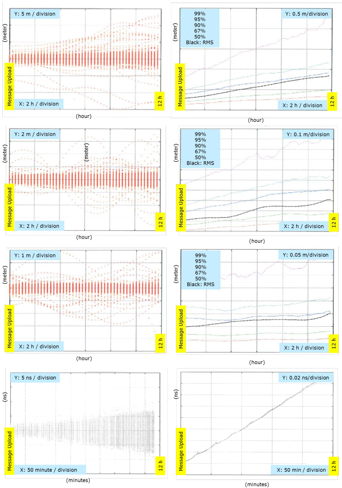
Figure 15 1st row: ALOE. 2nd row: ACOE. 3rd row RTOE. 4th row CE (in all cases over prediction time).
