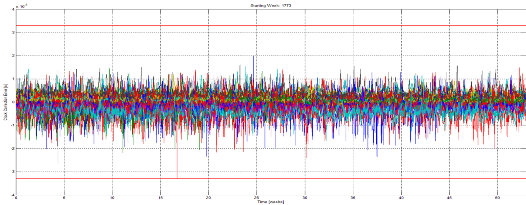
Figure 18. 1 st row: RTOE. 2 nd row: CE (red line corresponds to max observed error).
