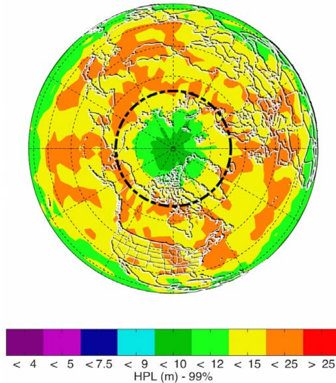
Figure 9: HPL for the Arctic Based on ARAIM with Dual Frequency GPS + Galileo
