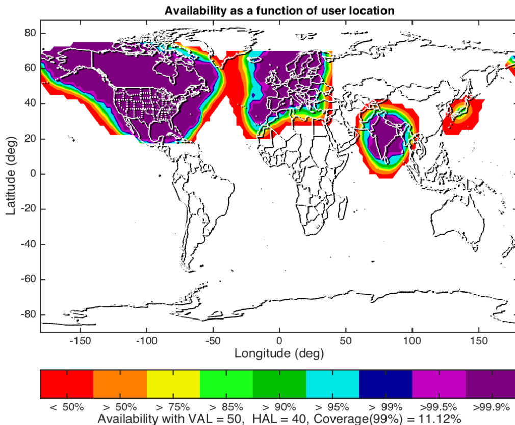
Figure 3: SBAS Coverage for LPV-200 in 2015
