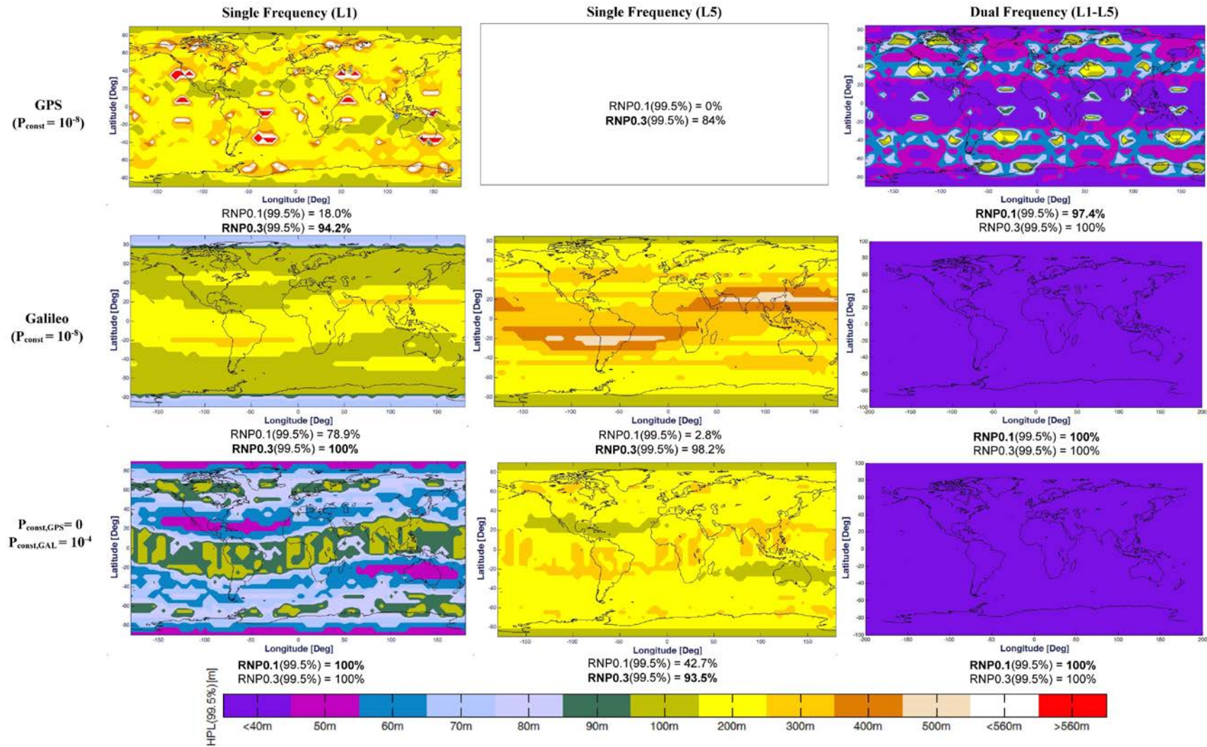
Figure 13: HPL(m)-99.5% map for the baseline constellation configuration with P_{sat} = 10^{-5} , b_{nom} = 0.75 m and \sigma_{URA} = 2.5 m
