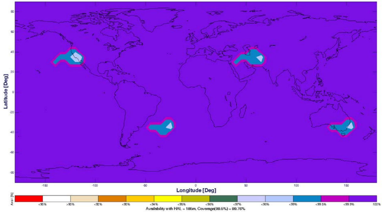
Figure 12: Availability map for the depleted constellation configuration and DFMC H-ARAIM, P_{const,GAL} = 10^{-4} , P_{const,GPS} = 0 , P_{sat} = 10^{-5} and \sigma_{URA} = 2.5 m
