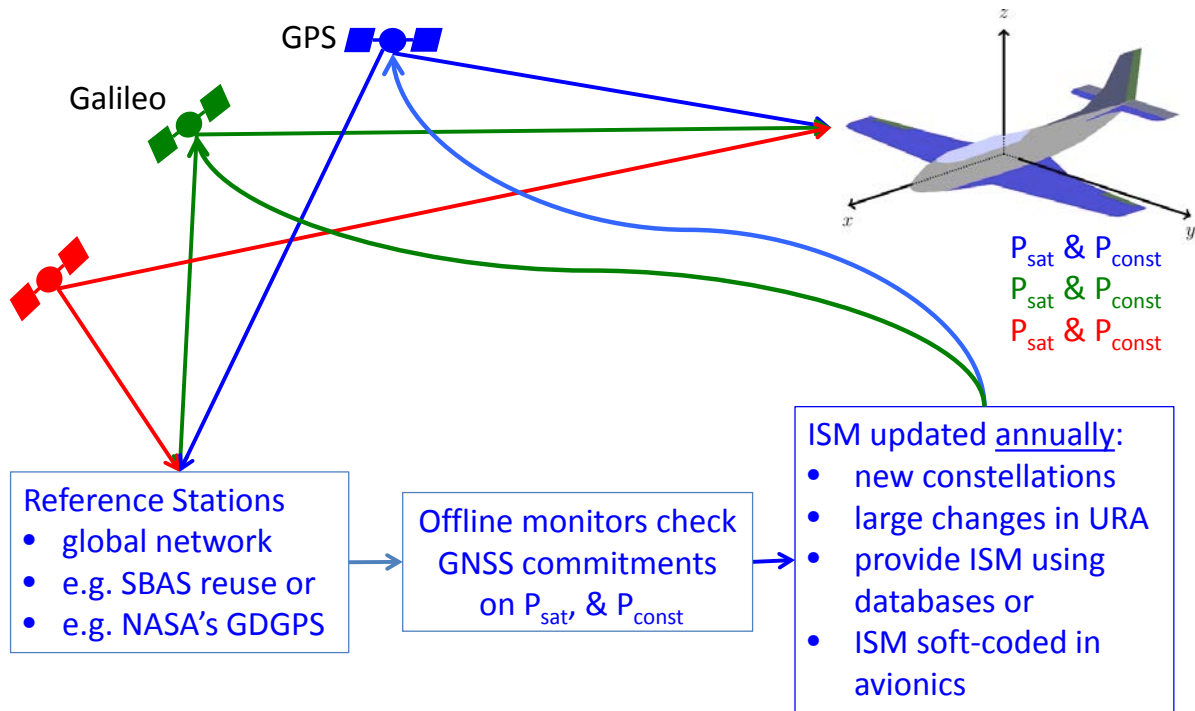
Figure 5: Horizontal ARAIM
