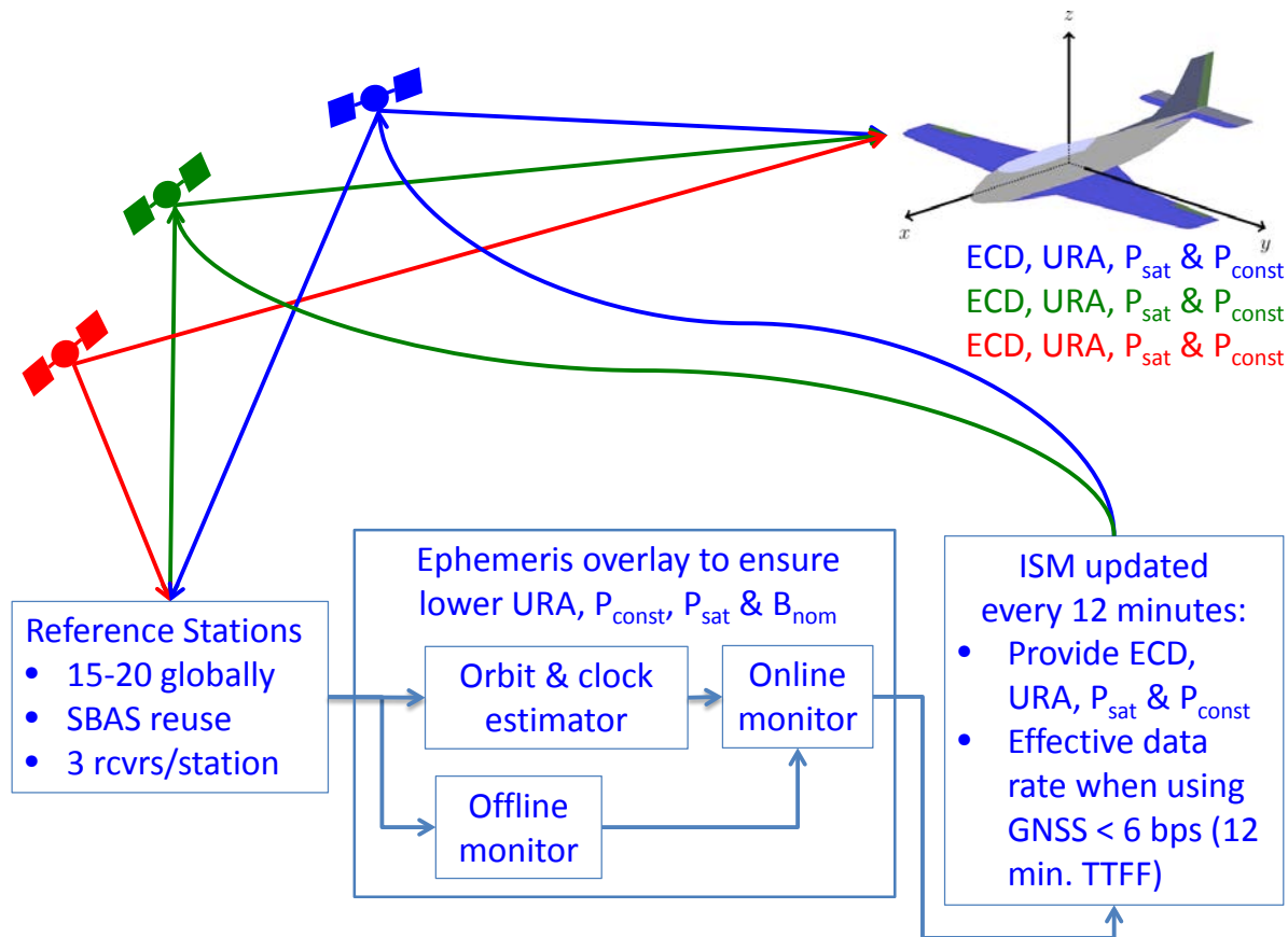
Figure 11: Online V-ARAIM replaces the Ephemeris & Clock (ECD) Generated by the Core Constellations
