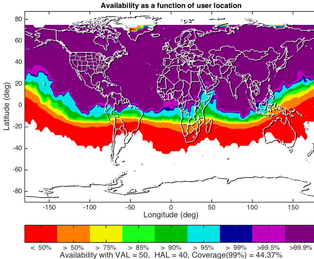
Figure 4: SBAS Coverage for LPV-200 in 2026
