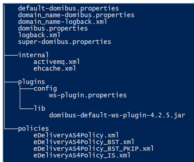
Figure 5 - Domibus configuration files
