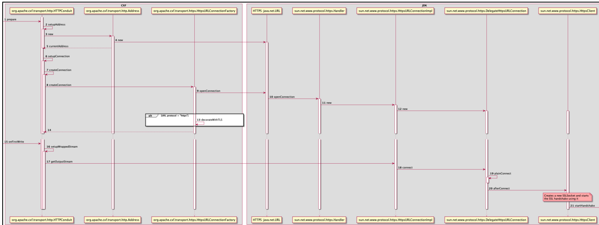
Figure 9 – SSL handshake
