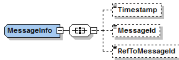
Figure 10 – MessageInfo type
