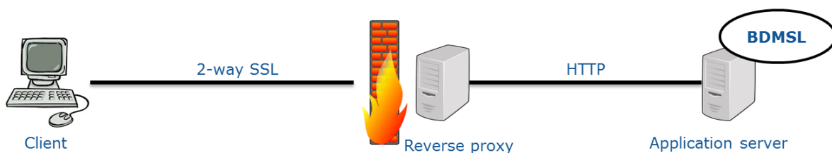
Figure 24 - Reverse proxy with SSL
