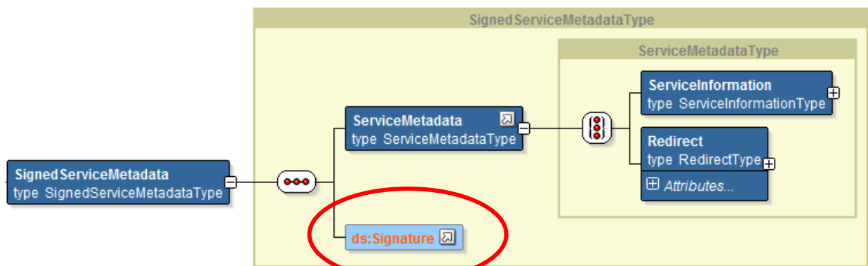
Figure 10- SignedServiceMetadata data model
