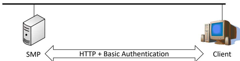
Figure 16- Basic authentication
