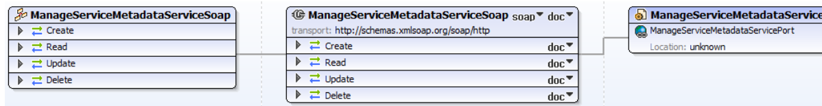
Figure 6 – WSDL ManageServiceMetadataService
