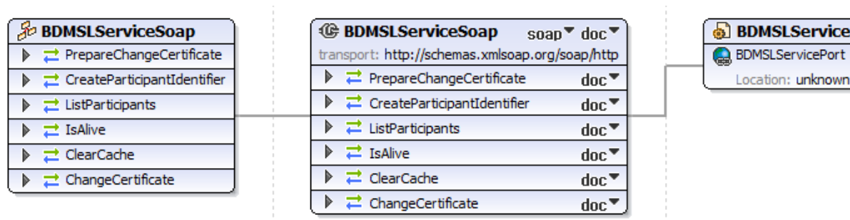
Figure 8 – WSDL BDMSLService
