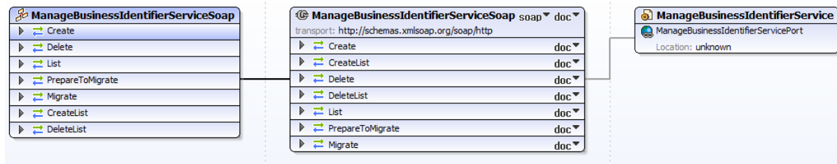
Figure 8 – WSDL ManageBusinessIdentifierService
