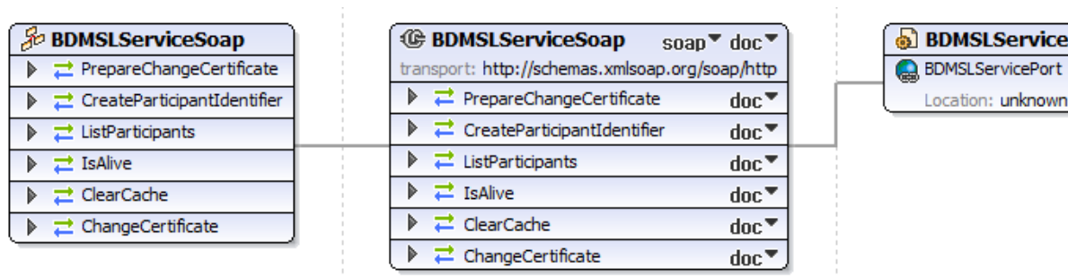
Figure 8 – WSDL BDMSLService
