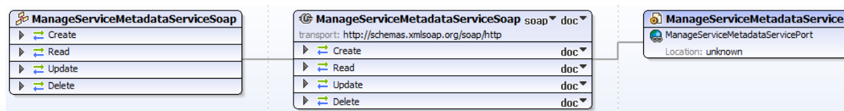
Figure 6 – WSDL ManageServiceMetadataService
