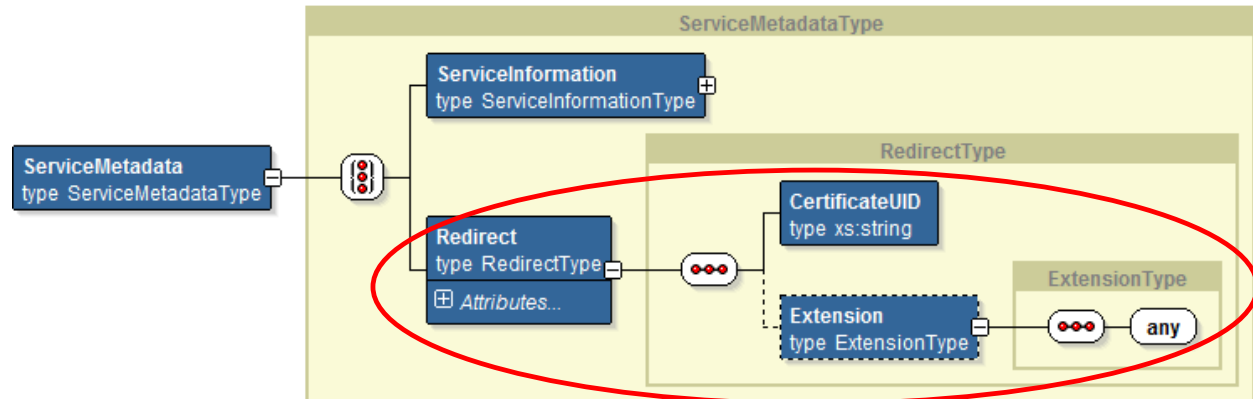
Figure 8- Redirect data model
