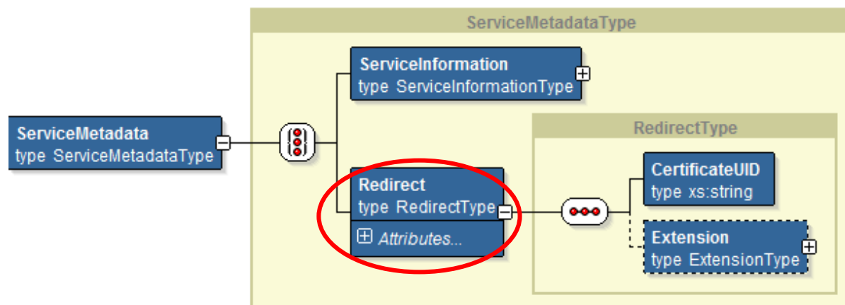
Figure 12- ServiceMetadata data model
