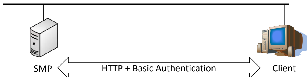
Figure 17- Basic authentication
