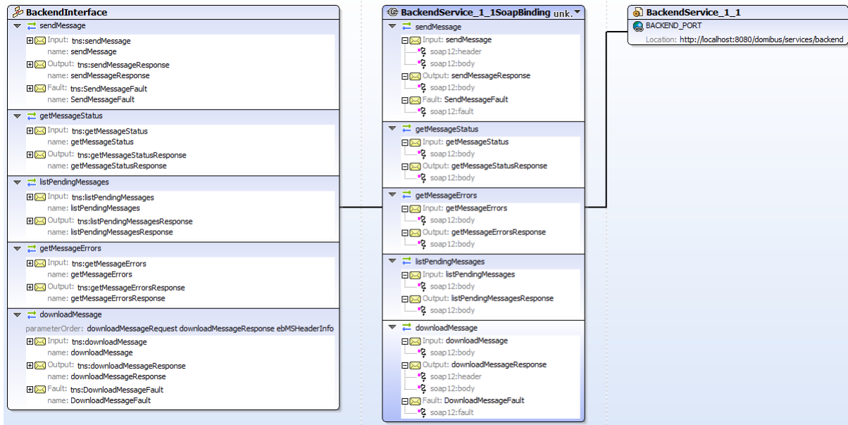
Figure 10 - WSDL model for Domibus 3.3-RC1
