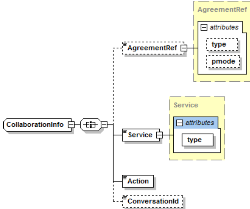
Figure 14 – CollaborationInfo type
