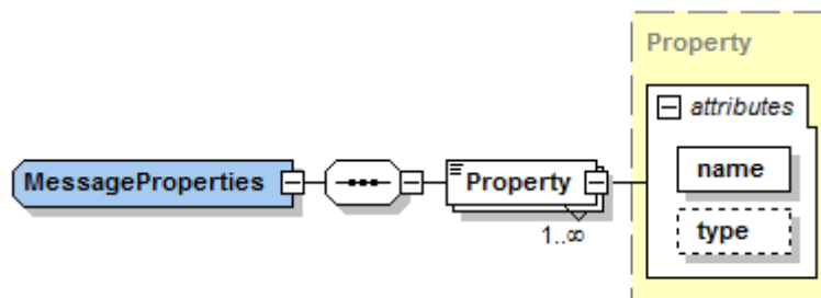
Figure 15 – MessageProperties type
