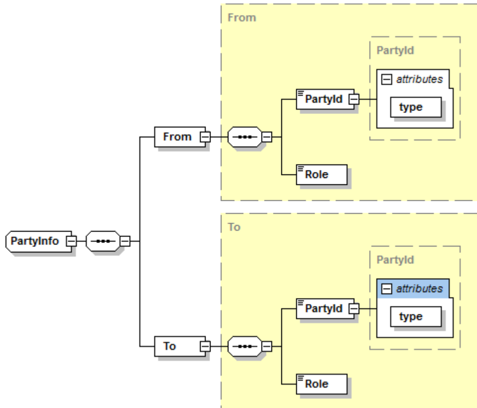
Figure 13 – PartyInfo type
