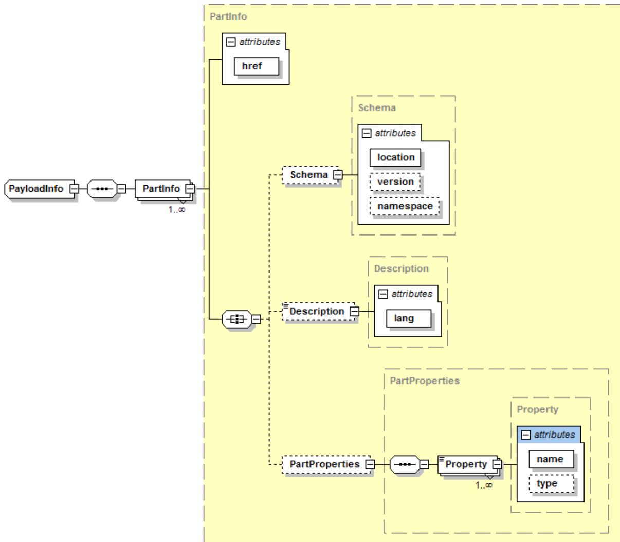
Figure 16 – PayloadInfo type
