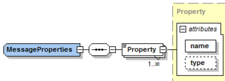
Figure 15 – MessageProperties type
