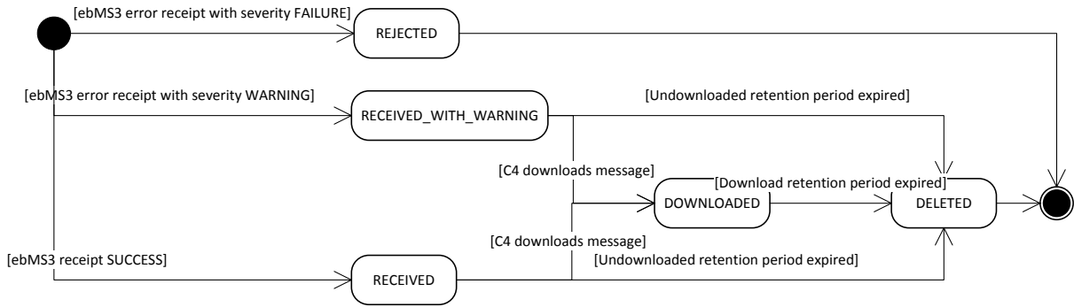
Figure 5 - State machine of C3
