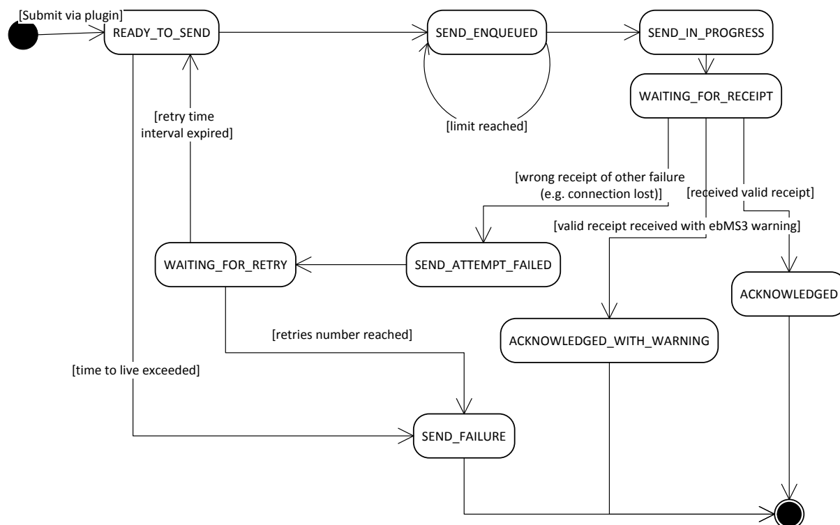
Figure 4 – State machine of C2
