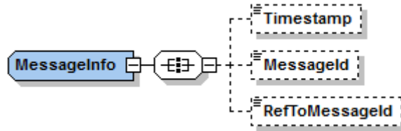
Figure 11 – MessageInfo type
