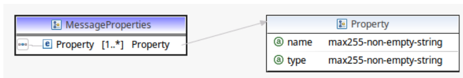
Figure 9 - MessageProperties schema
