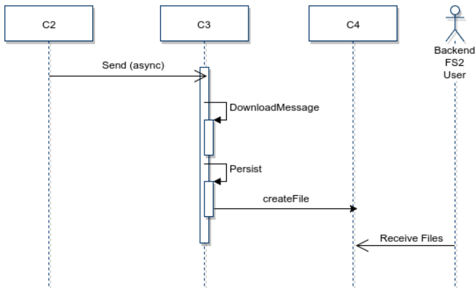
Figure 12 - Receive Files sequence diagram
