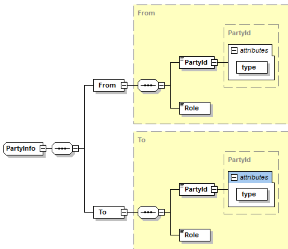
Figure 12 – PartyInfo type
