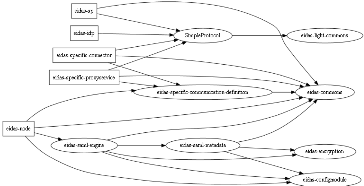
Figure 2: Component dependencies
