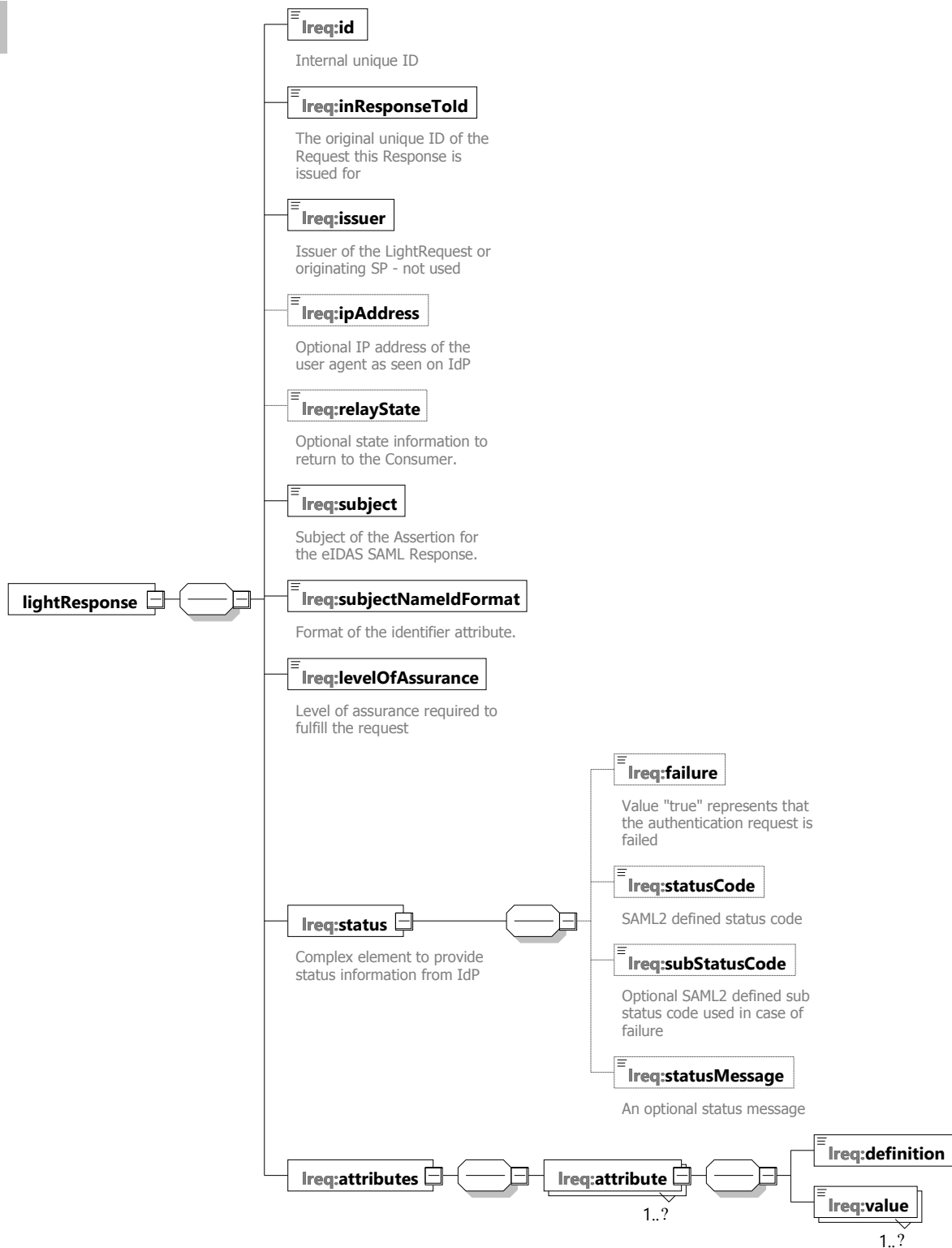
Figure 14: Simplified XML LightResponse schema
