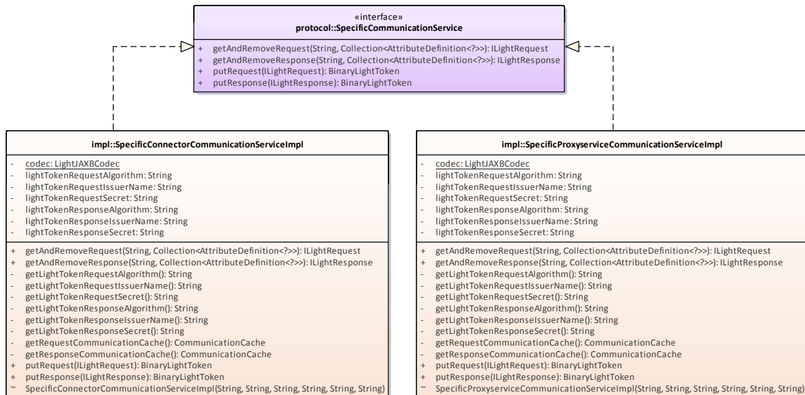
Figure 10: SpecificCommunicationService
