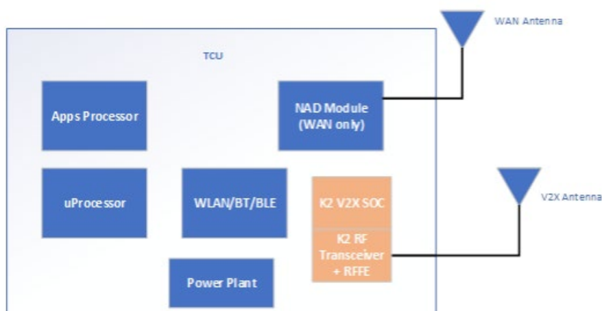
Figure 3 – Standalone C-V2X communications systems
