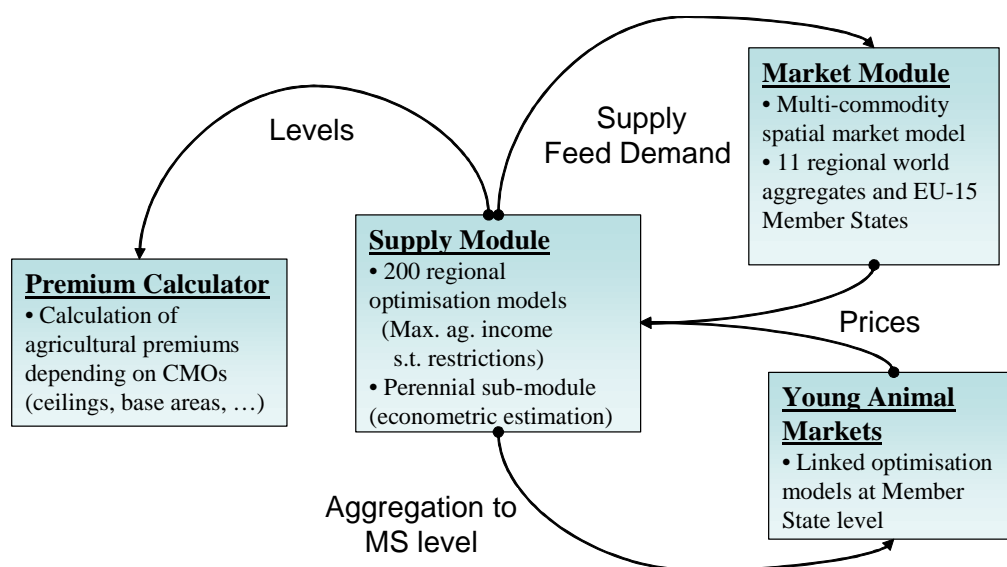
Figure 2. Link of modules in CAPRI
