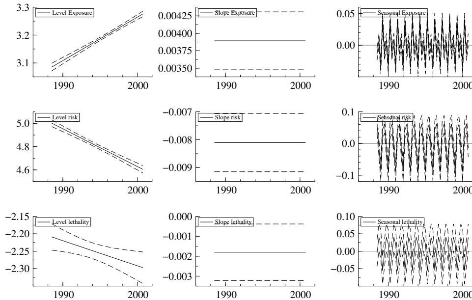
Figure 3.5. Smoothed trend, slope and seasonal components of multivariate linear regression for the whole of the Netherlands, including 95% confidence limits.
