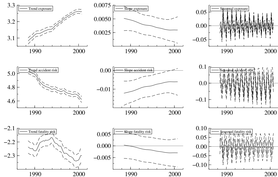
Figure 3.2. Smoothed trend, slope and seasonal components for the whole of the Netherlands, including 95% confidence limits.
