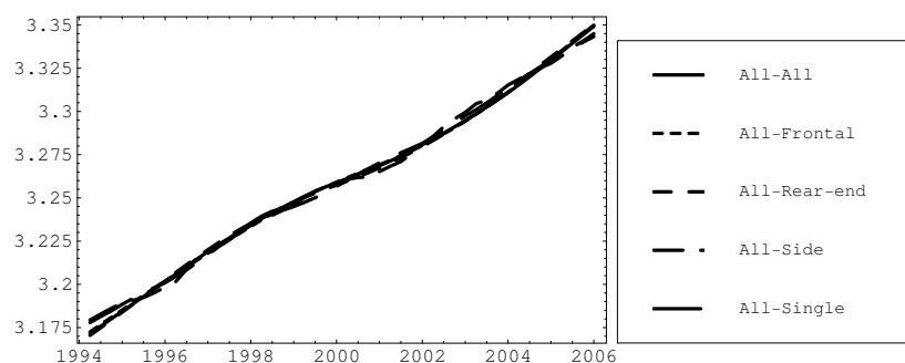
Figure 5.1. Trends of the latent variable for total exposure.
