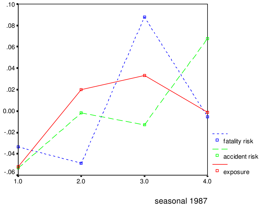
Figure 2.3.a Quarterly seasonals in 1987 for the whole of France.
