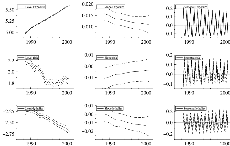
Figure 4.4. Smoothed trend, slope, and seasonal components for French motorways, including 95% confidence limits.
