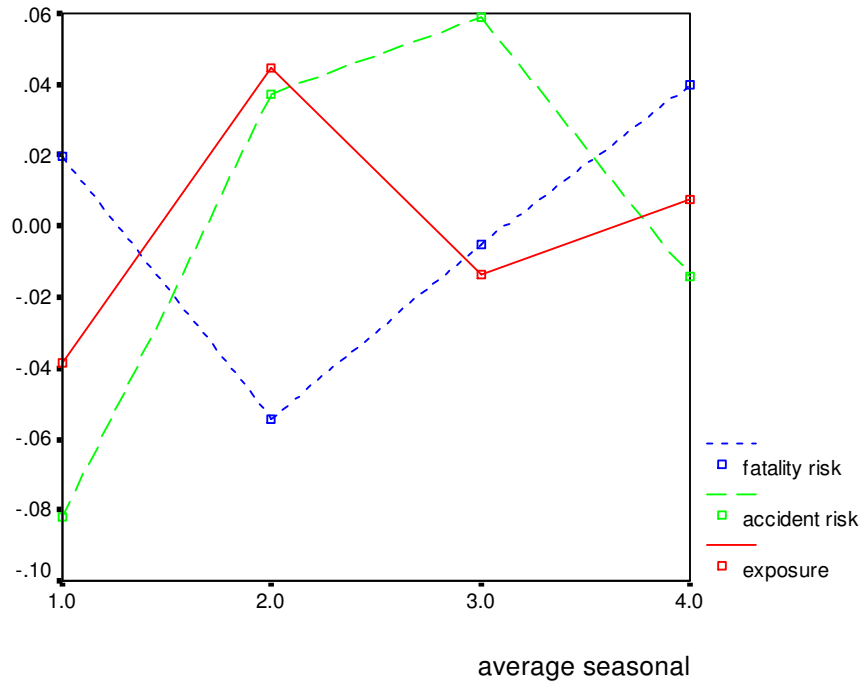
Figure 3.3.b. Average quarterly seasonals for the whole of the Netherlands.
