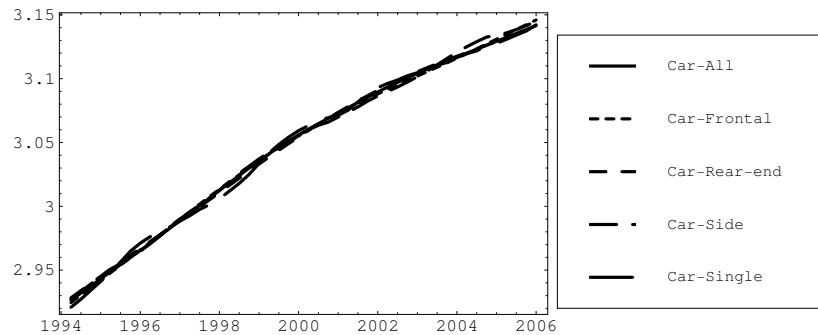
Figure 5.4. Trends of latent variable for Car-car exposure.
