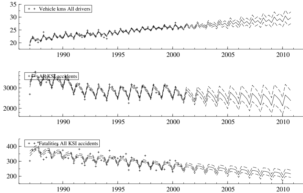
Figure 3.7. Forecasts of stochastic three-level model applied to the whole of the Netherlands, including 68% confidence limits.
