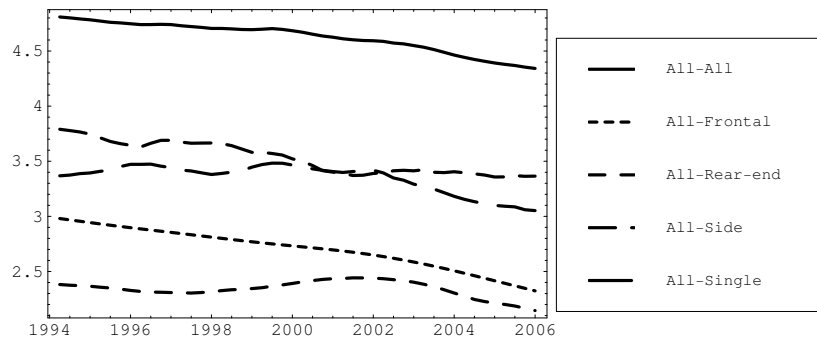
Figure 5.2. Trends of latent variable for total accident risk: KSI accidents per driver kilometre.
