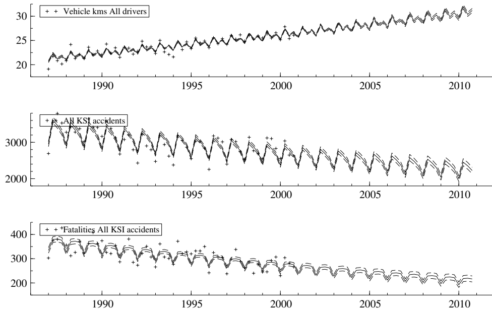
Figure 3.6. Forecasts of deterministic three-level model applied to the whole of the Netherlands, including 68% confidence limits.
