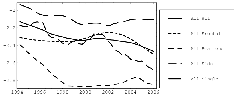
Figure 5.3. Trends of latent variable for total severity risk: fatalities per KSI accident.
