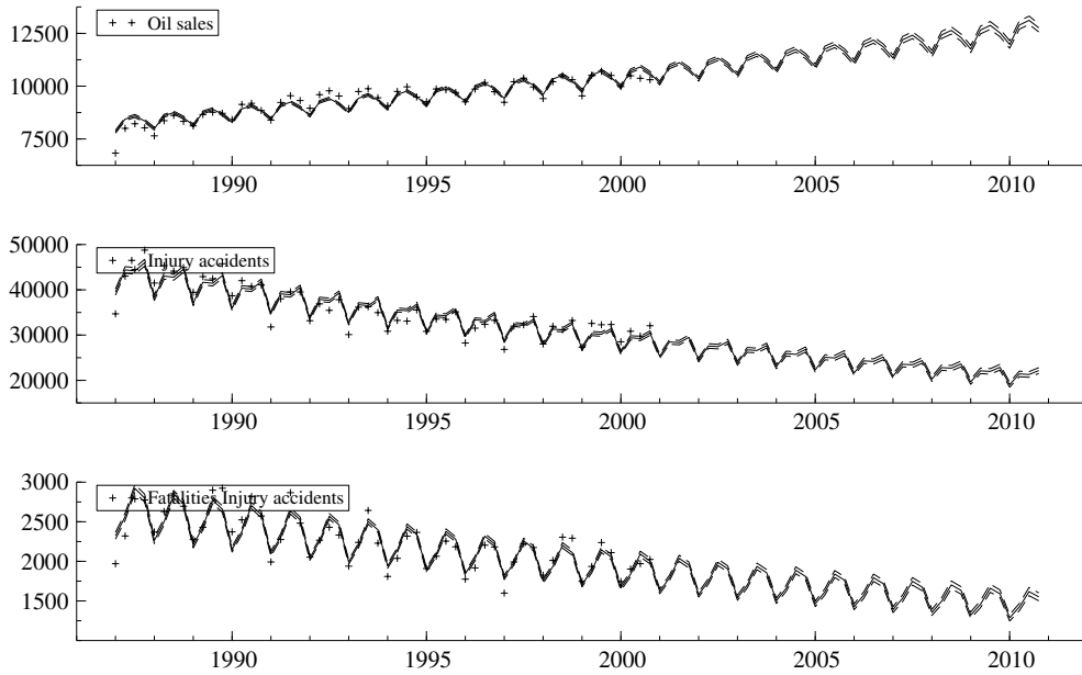
Figure 2.6. Forecasts of deterministic three-level model applied to the whole of France, including 68% confidence limits.
