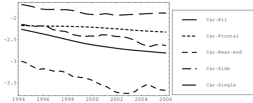
Figure 5.6. Trends of latent variable for Car-car fatality risk: fatalities per KSI accident.
