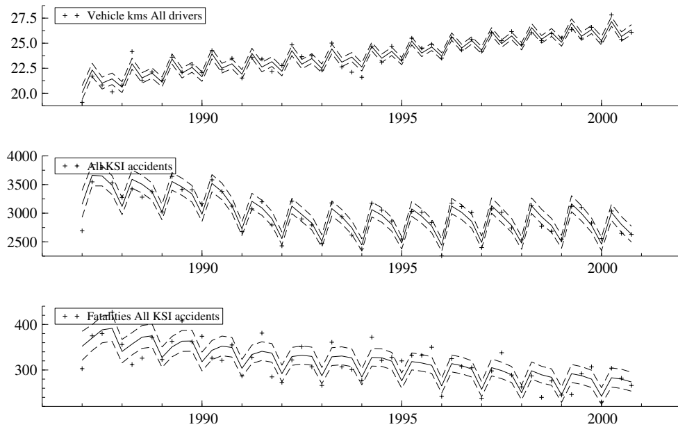
Figure 3.1. Smoothed predictions for quarterly vehicle kilometres, KSI accidents, and fatalities for the whole of the Netherlands, including 95% confidence limits.
