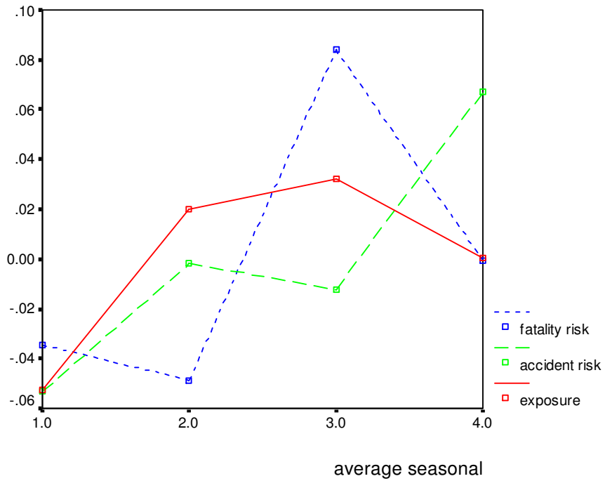
Figure 2.3.b Average quarterly seasonals for the whole of France.
