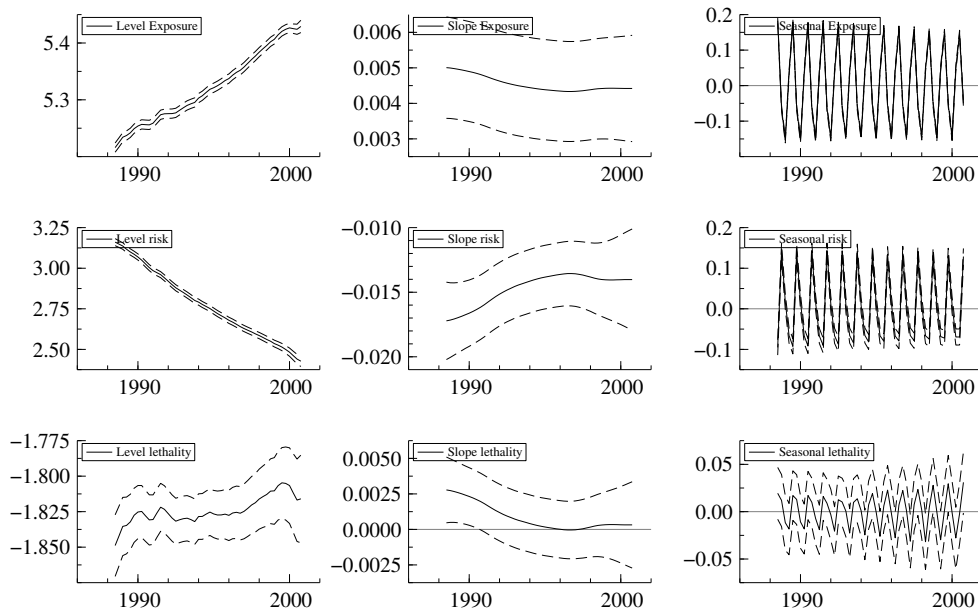
Figure 4.2. Smoothed trend, slope, and seasonal components for French main roads, including 95% confidence limits.
