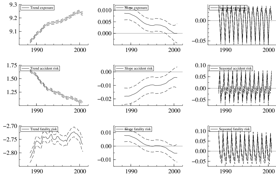
Figure 2.2. Smoothed trend, slope and seasonal components for the whole of France (uninterrupted lines), including 95% confidence limits (between dashed lines).
