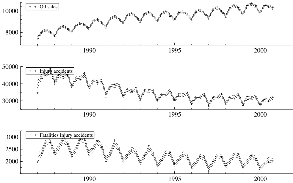
Figure 2.1. Smoothed predictions (uninterrupted lines) for quarterly oil sales, injury accidents, and fatalities for the whole of France, including 95% confidence limits (between dashed lines).
