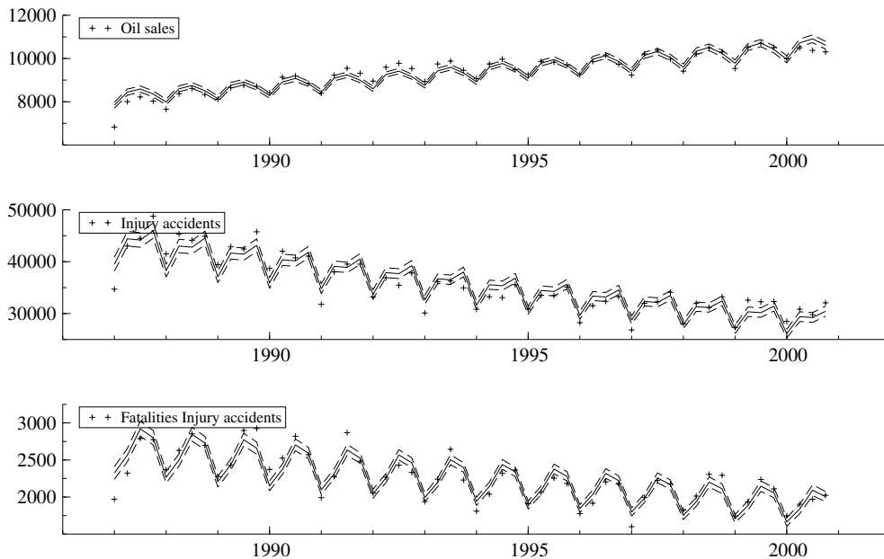
Figure 2.4. Smoothed predictions for oil sales, injury accidents, and fatalities of multivariate linear regression for the whole of France, including 95% confidence limits.
