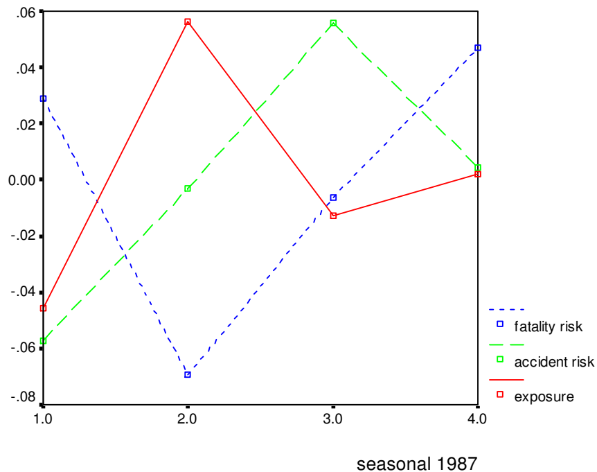
Figure 3.3.a. Quarterly seasonals in 1987 for the whole of the Netherlands.
