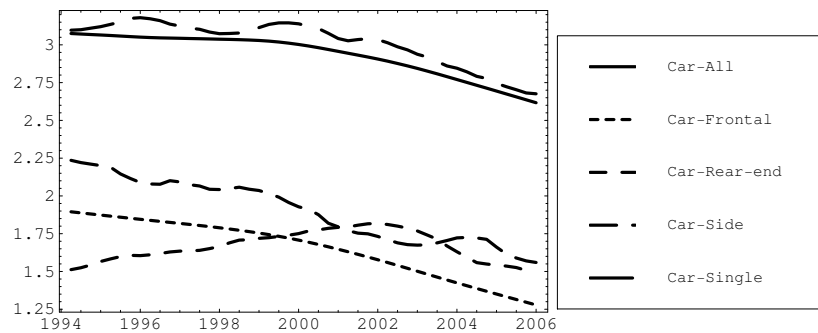
Figure 5.5. Trends of latent variable for Car-car accident risk: KSI accidents per driver kilometre.
