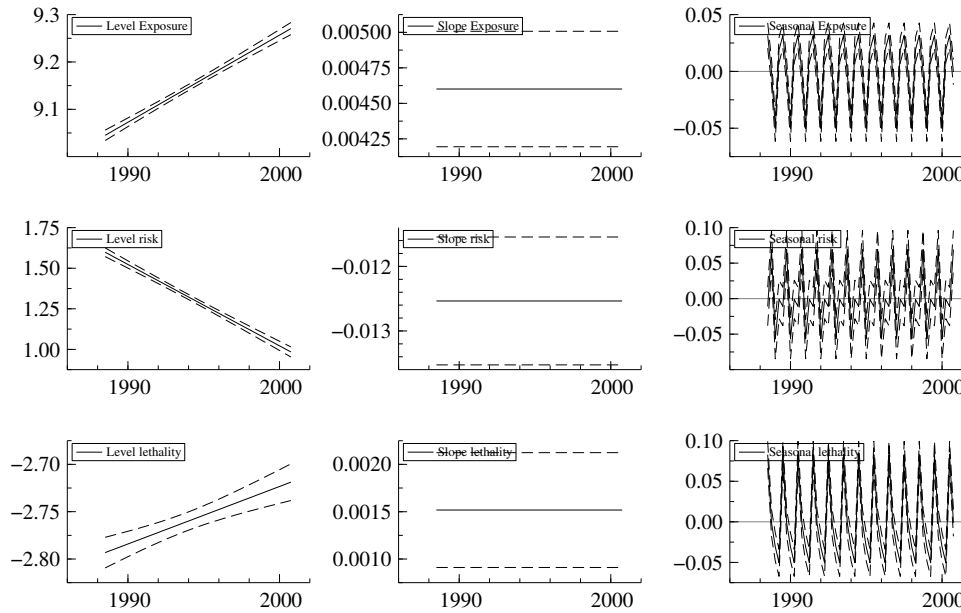
Figure 2.5. Smoothed trend, slope and seasonal components of multivariate linear regression for the whole of France, including 95% confidence limits.
