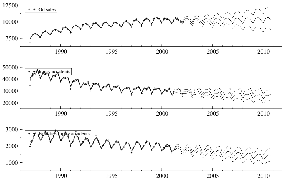
Figure 2.7. Forecasts of stochastic three-level model applied to the whole of France, including 68% confidence limits.
