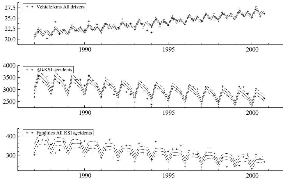
Figure 3.4. Smoothed predictions for quarterly vehicle kilometres, KSI accidents, and fatalities of multivariate linear regression for the whole of the Netherlands, including 95% confidence limits.
