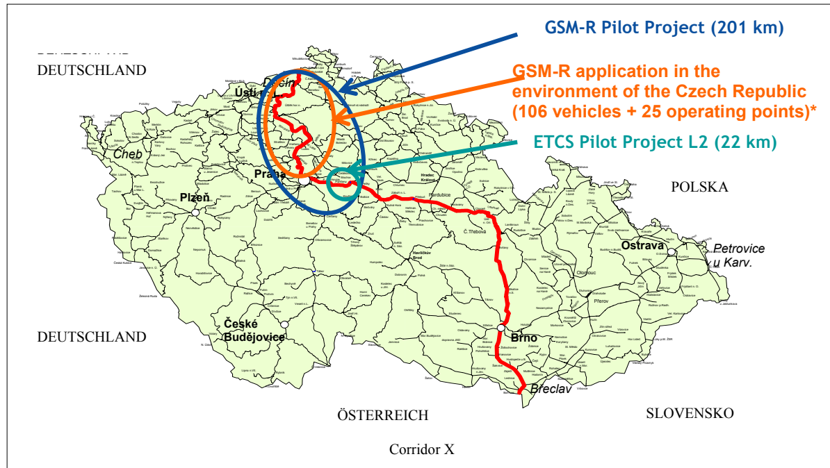
Fig. 3 – ERTMS/GSM-R, ETCS pilot projects and GSM-R application
