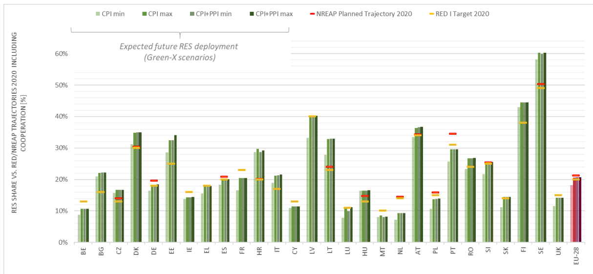
Figure 4. Expected renewable energy shares in 2020 vs. 2020 RED targets and 2020 planned (NREAP) targets, including cooperation mechanisms (MS, %). Source: Navigant 2019.
