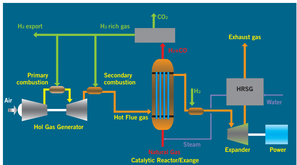
SP1-WP1: Hygensys: the process concept
