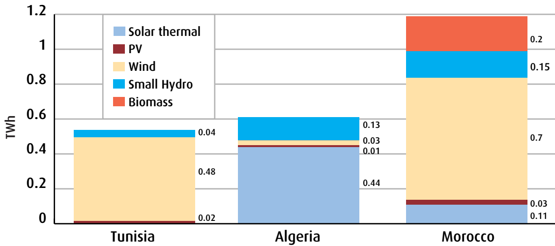
RENEWABLE ENERGY SOURCE (EXCLUDING LARGE HYDRO)-BASED POWER GENERATION IN 'MODRES 2010 SCENARIO'(IN TWh) (by source and country)
