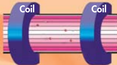
Plasma with magnetic field
