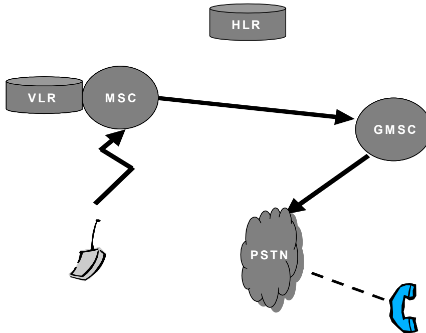
Diagram A1.2: Call Origination
