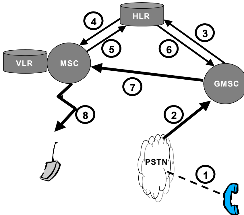
Diagram A1.3: Call Termination
