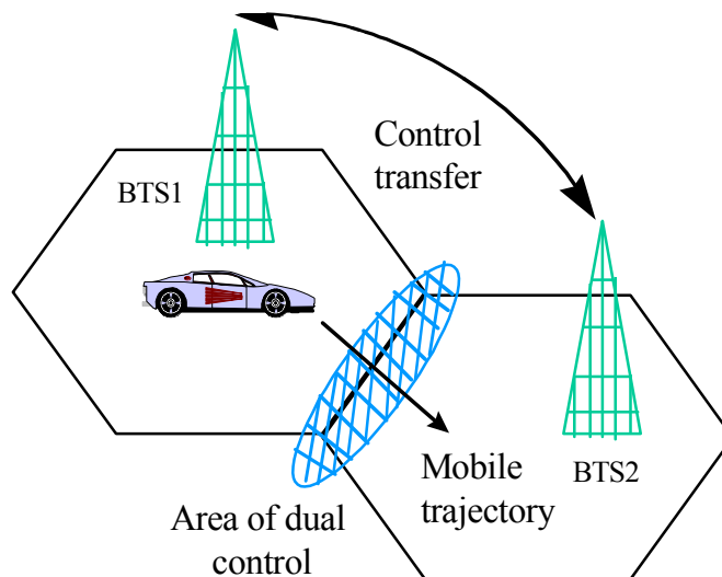
Figure 3.3: Handover Procedure
