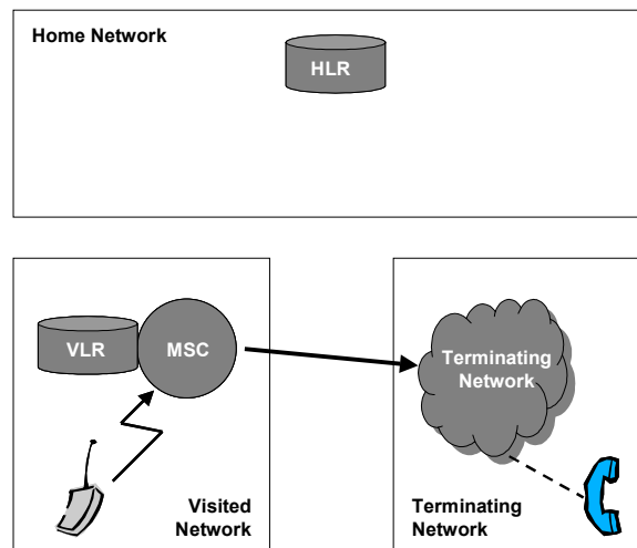
Diagram A1.7: Roaming subscriber originating a call
