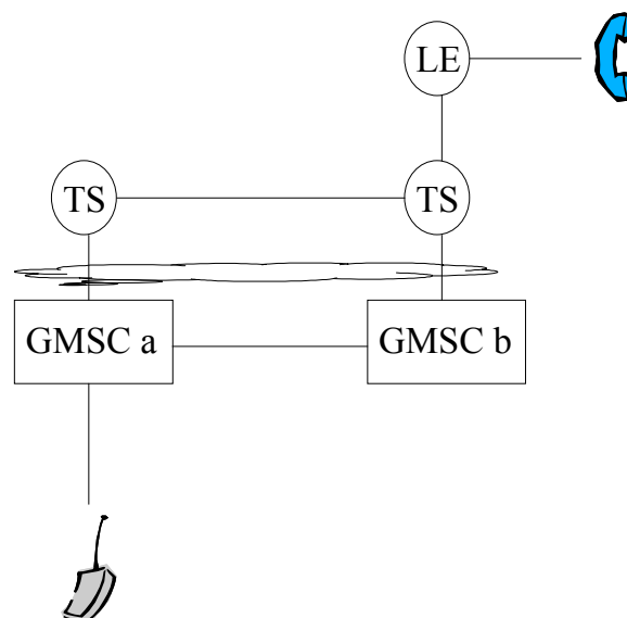
Diagram A1.5: Fixed-Mobile Calls
