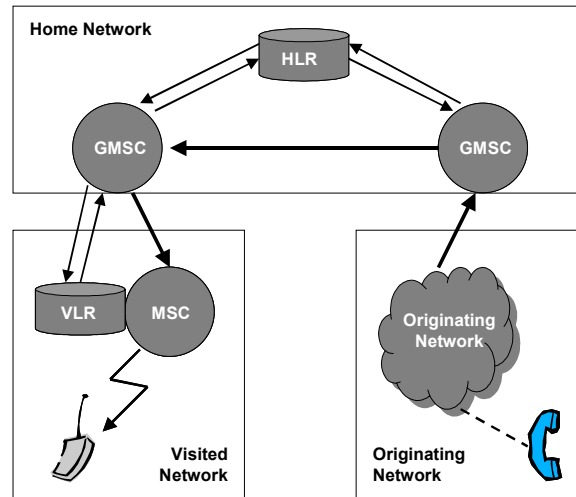
Diagram A1.8: Terminating a Call to a Roaming Customer
