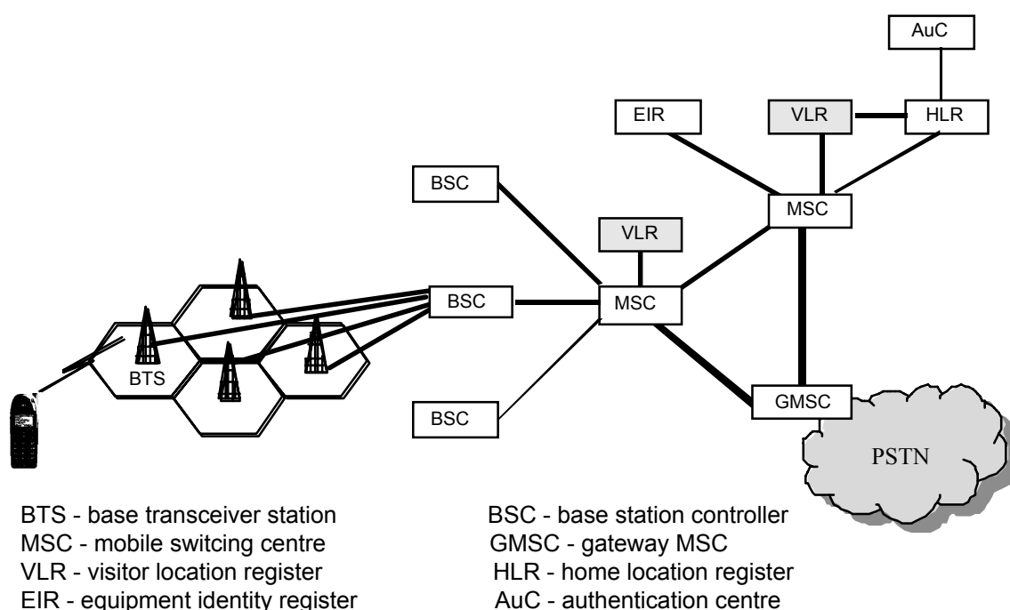
Figure 3.1: Structure of the GSM Mobile System
