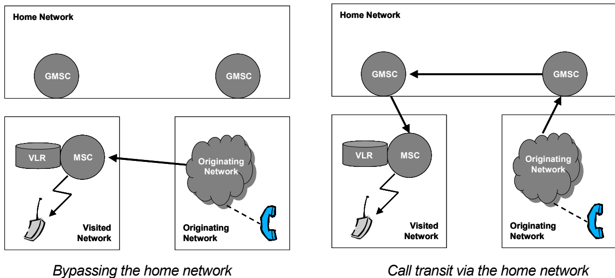
Diagram 8.1: Alternative call transit routes for call termination
