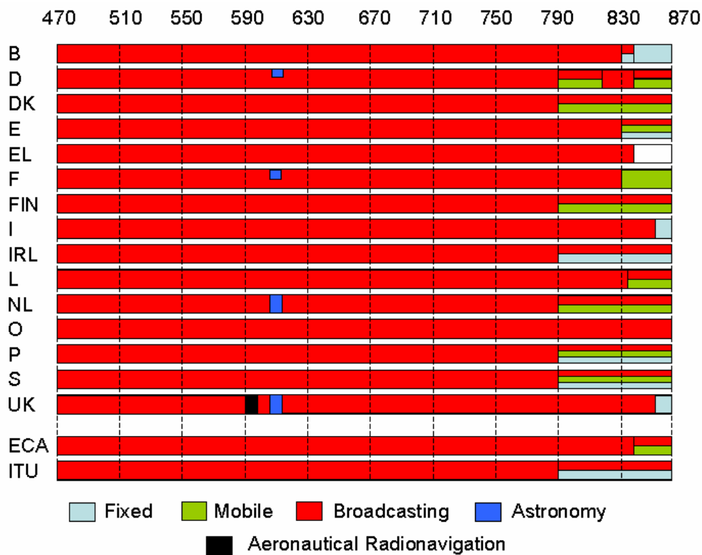
Figure D.5: Primary allocations and protected services in UHF Bands IV and V
