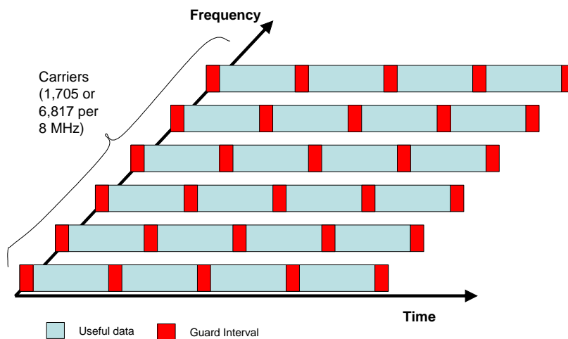
Figure E.6 DVB-T Signal in time and frequency domains
