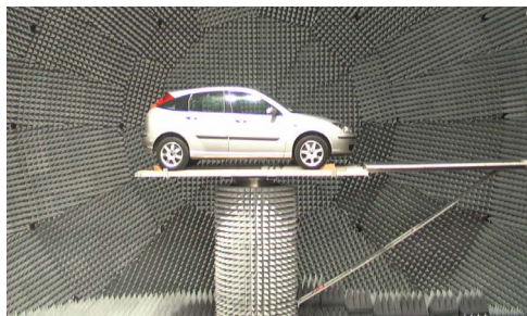
MIMO antenna measurement
