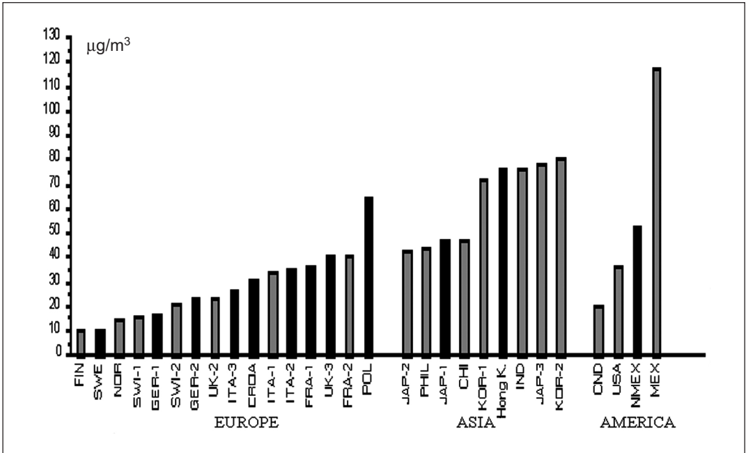
Figure 4.1. Residential mean NO 2 concentrations in different countries
