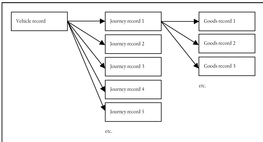
Figure 1: Data structure
